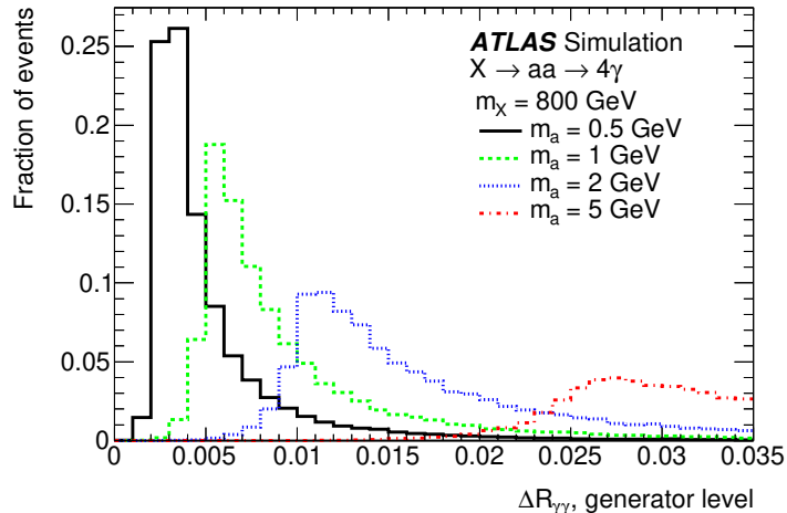
Figure 2: The distribution of \Delta R_{\gamma\gamma} , the angular separation between two photons that are reconstructed as a single photon-jet in the ATLAS detector, for the benchmark signal scenario for the process X \rightarrow aa \rightarrow 4\gamma , using simulated signal samples at generator level. The distribution has a peak at \sim 4 \times m_a/m_X and a long tail on the right side. For the values of m_X and m_a presented in the figure, \Delta R_{\gamma\gamma} is smaller than or comparable in size to an EM cluster.
