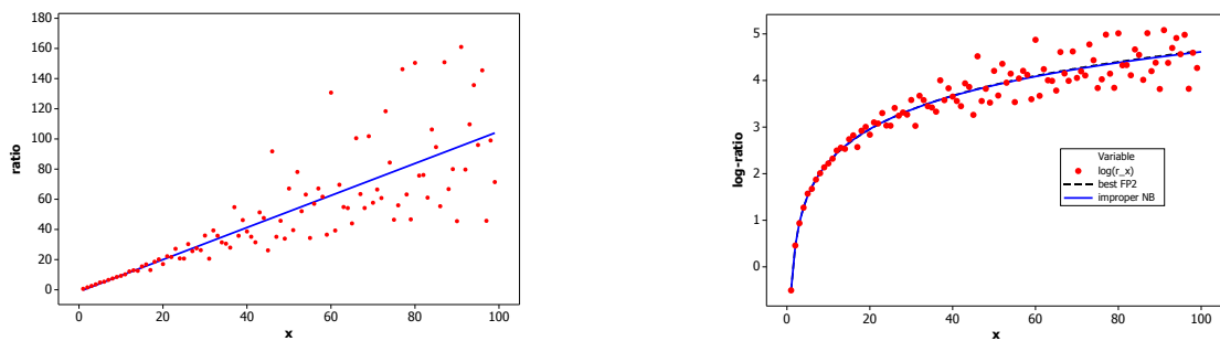
Figure 2. Word frequency count of Shakespeare's works: ratio plot r_x against x , (left panel), improper negative binomial distribution (solid) and best fractional polynomial of order 2 (dashed), (right panel)
