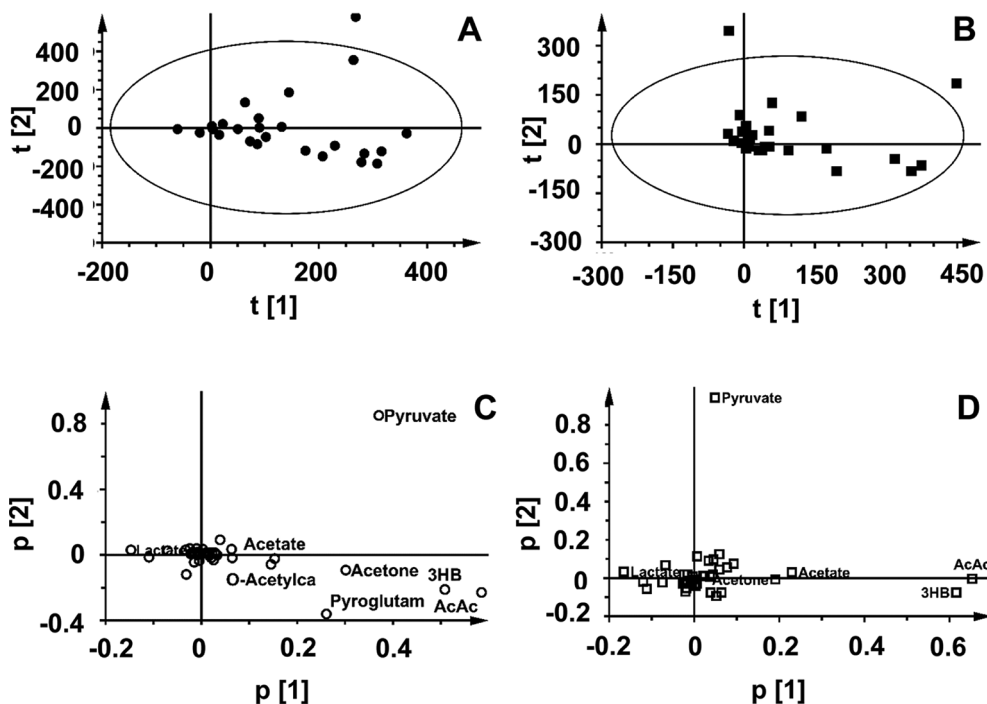
Figure 3 Change percentage induced by angioplasty: (after)–(before)/(before) × 100. Principal component analysis score and loading plots of arterial (A–C) and venous (B–D) serum samples.
