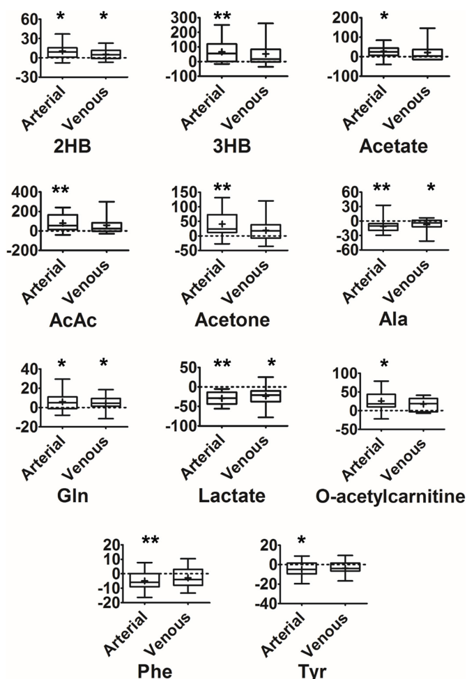
Figure 4 Change percentage induced by angioplasty in arterial (A) and venous (V) serum metabolites. Boxes denotes IQR, lines denotes median, whiskers denotes 5th and 95th percentile, +denotes the average. *P<0.01; **P<0.001. 2HB, 2-hydroxybutyrate; 3HB, 3-hydroxybutyrate; Ala, alanine; Gln, glutamine; Lys, lysine; Phe, phenylalanine; Tyr, tyrosine; Val, valine.
