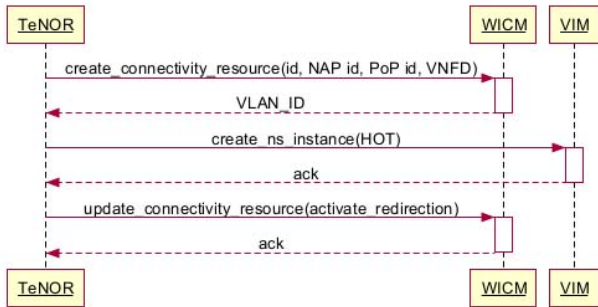
Fig. 9. High-level TeNOR NS Provisioning Sequence Diagram.
