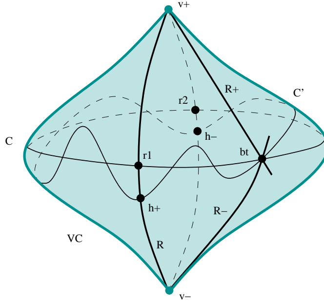
FIGURE 4. The double cover Y_0 of the quartic cone V_0 .
