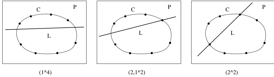
FIGURE 2. Hyperelliptic degenerations in the strata (1^4), (2, 1^2), (2^2) .
