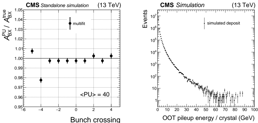
Figure 10. Left: bias in the out-of-time amplitude estimated by the multifit algorithm as a function of BX, for the bunch crossings -5 \leq BX \leq +4 . The in-time interaction corresponds to BX = 0 in the figure. The bias is estimated as the mode of the distribution of the ratio between the measured and the true energy. Only statistical uncertainties are shown. Right: energy spectrum in an ECAL barrel crystal, at \eta \approx 0 .
