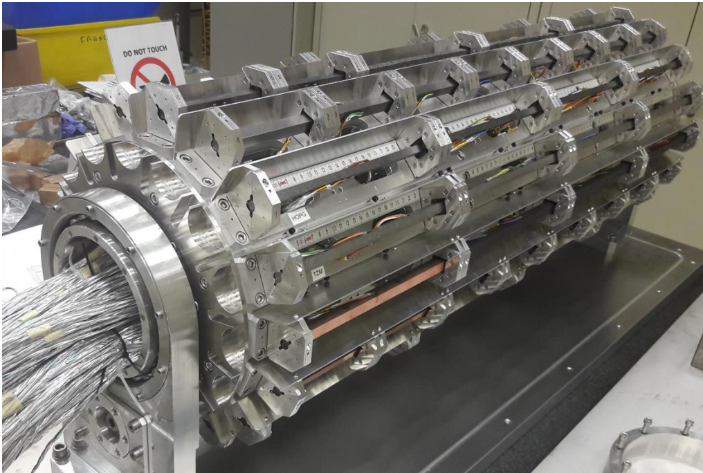
Figure 2: Rotatable barrel with mounted target stations. Note shielded cables for on-board instrumentation.
