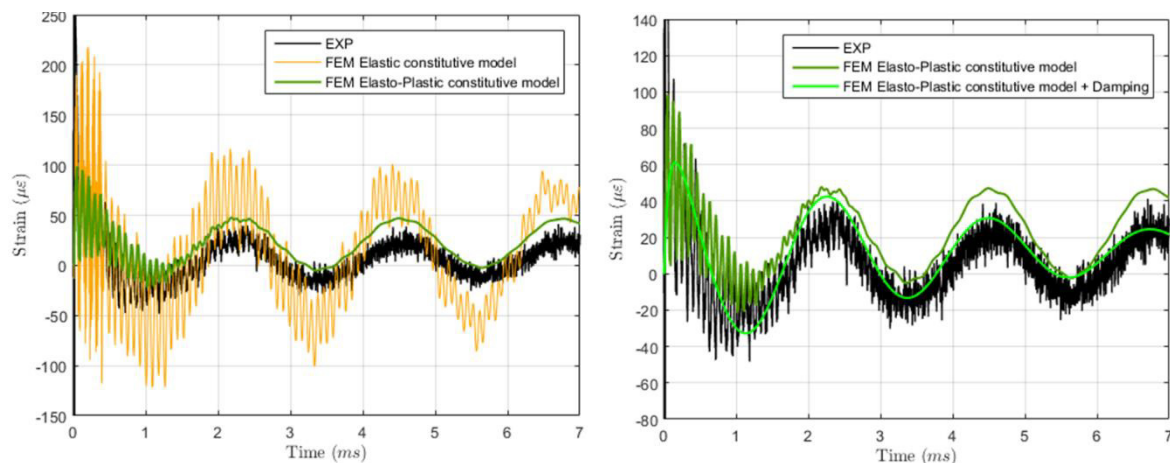
Figure 5: Flexural oscillations in the most loaded specimen of CuCD-grade 1. Numerical/experimental comparison.
