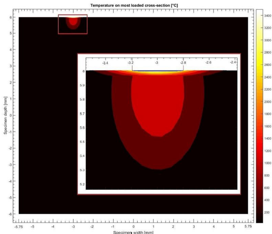
Figure 7: Temperature distribution induced on the most loaded cross section of Mo-coated CFC by a 288 b impact.
