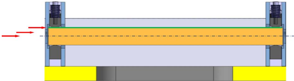
Figure 3: Typical specimen configuration, showing a scheme of beam impacts: centred, offset and grazing on coated surface (in green).
