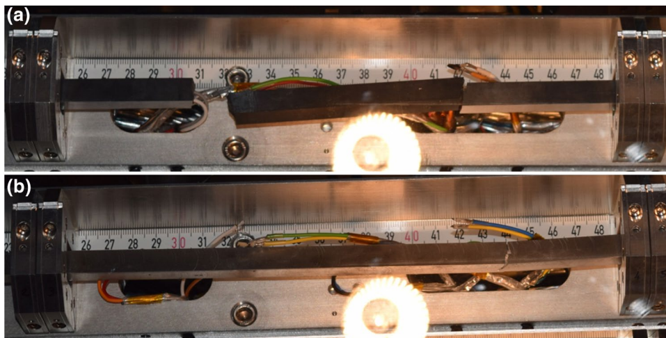
Fig. 31 The beam-induced failure of the second SiC sample of line 5 and of the second TZM sample of line 14, impacted by a 36 bunches-pulse with 1.18 \times 10^{11} p/b and \sigma = 0.5 mm and by a 12-bunches pulse with 1.33 \times 10^{11} p/b and \sigma = 2 mm, respectively
