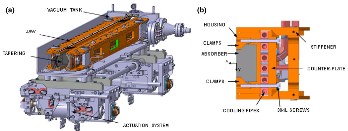
Fig. 1 Cutaway drawing of a HL-LHC secondary collimator (a) and transverse cross-section of the collimator jaw (b)
