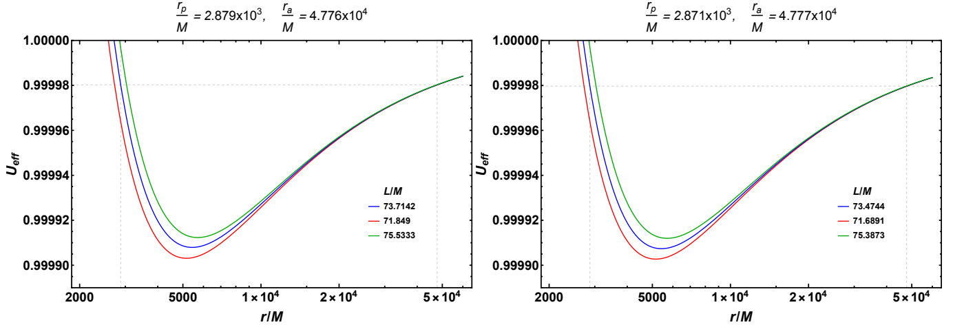
Fig. C.3. Effective potential U_{\text{eff}} given by Eq. (C.19) for selected values of the conserved angular momentum L . Left: massive BH case, i.e., Schwarzschild solution, g_{00} = 1 - 2M/r . Right: DM case; g_{00} obtained from numerical integration of the general relativistic equilibrium equations of the extended RAR model for a fermion mass mc^2 = 56 keV, see Appendix A for details. Imposing a bound orbit within given values of the pericenter and apocenter (vertical dashed lines), in this example, r_p/M = 2.976 \times 10^3 and r_a/M = 4.714 \times 10^4 , respectively, implies a unique solution of E (dashed horizontal value) and L (value associated with the blue curve). In this example, the adopted mass of the massive BH for the Schwarzschild solution is M_{\text{BH}} = M = 4.075 \times 10^6 M_{\odot} , and for the mass of the DM RAR core, it was set to M_c = 3.5 \times 10^6 M_{\odot} .
