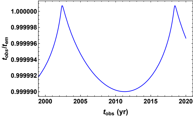
Fig. C.2. Ratio t_{\text{obs}}/t_{\text{em}} as given by Eq. (C.14), calculating Z(t_{\text{obs}}) with Eq. (C.9c), for the best-fit model parameters of the BH model Table 1, derived assuming Eq. (C.15).
