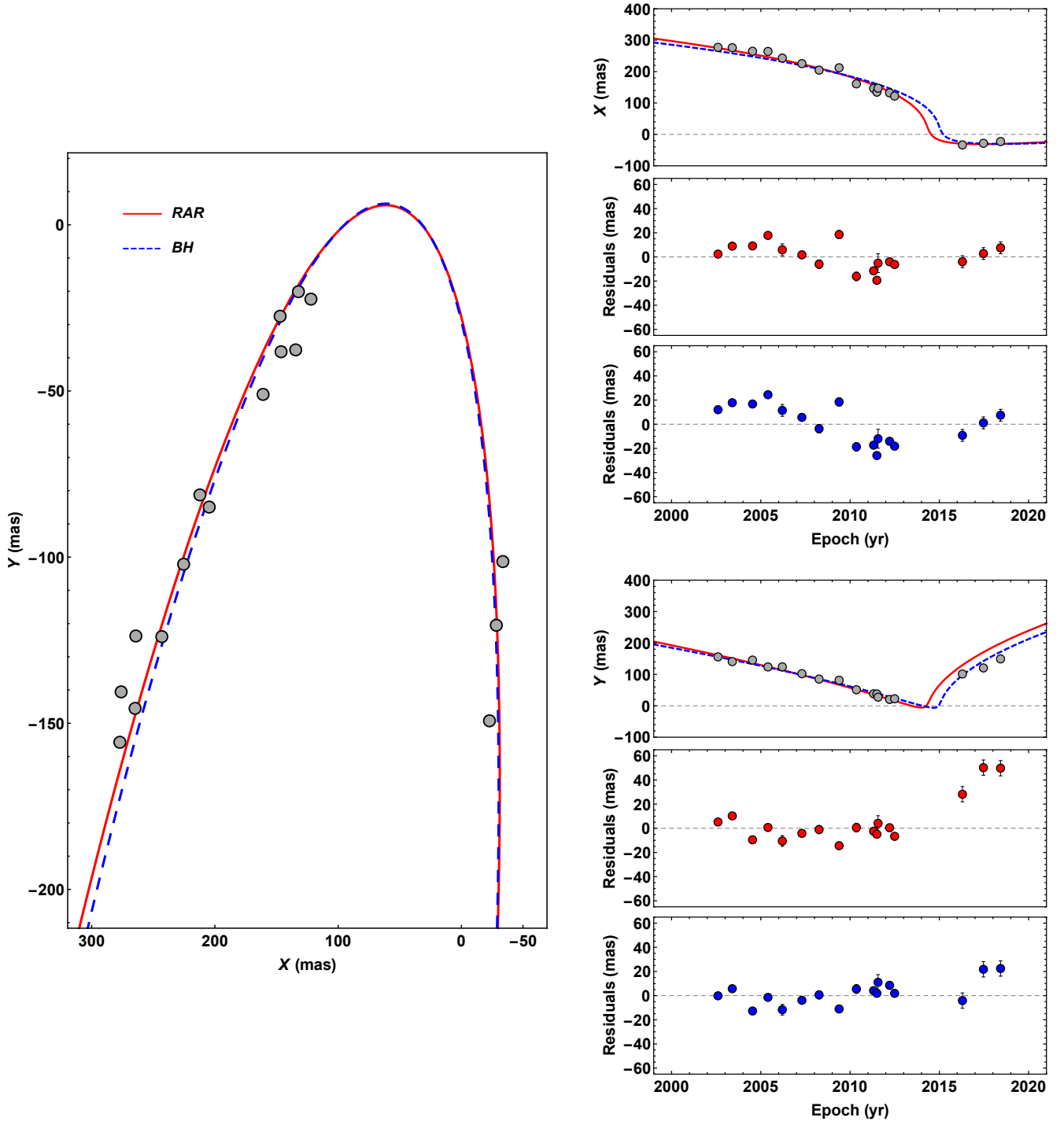
Fig. 4. Theoretical and observed orbit of G2 around Sgr A*. Left panel: orbit ( X vs. Y ), right panel: X and Y position as a function of time and the respective residuals of the best-fit for each model. The theoretical models are calculated by solving the equations of motion of a test particle in the gravitational field of (1) a Schwarzschild BH of 4.075 \times 10^6 M_{\odot} (dashed blue curves), and (2) the DM distribution obtained from the extended RAR model for 56 keV fermions (red curves). The mass of the quantum core in the RAR model is 3.5 \times 10^6 M_{\odot} . Table 1 shows the parameters of each model. The observational data are taken from Phifer et al. (2013) , Plewa et al. (2017) , and Gillessen et al. (2019) .
