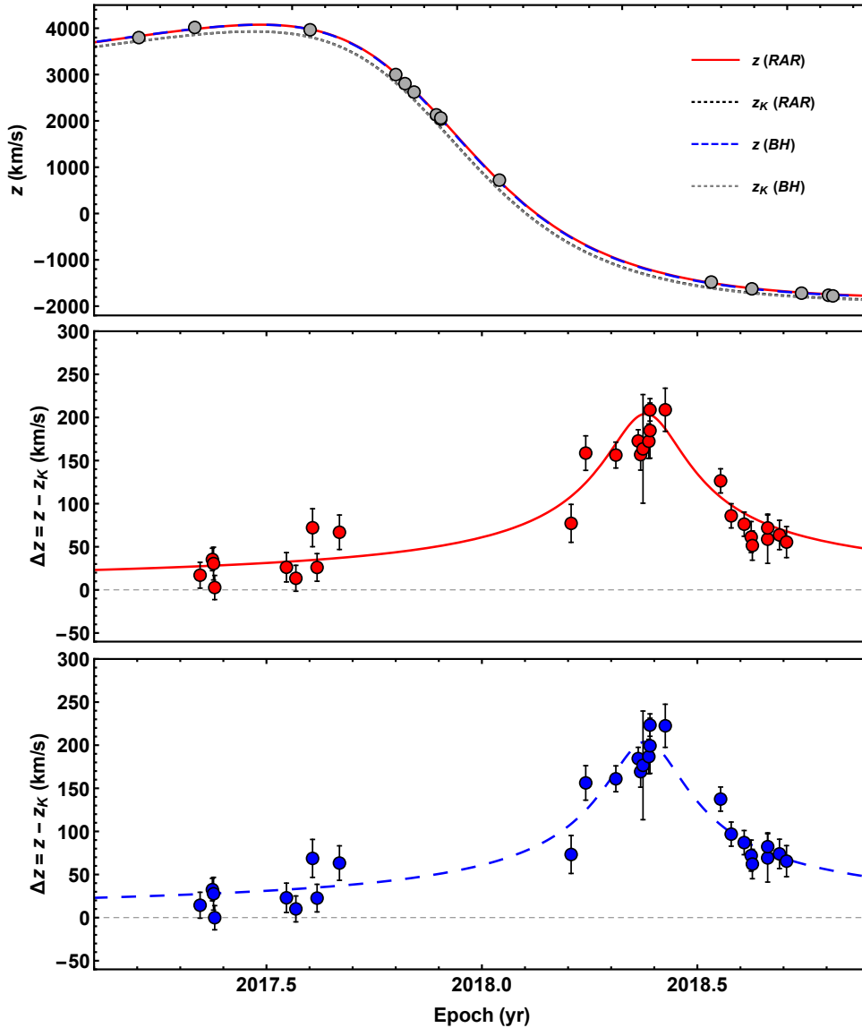
Fig. 6. Redshift function z (top panel) and redshift function “excess” (middle panel for the RAR model and lower panel for the central massive BH model) with respect to the Keplerian (Newtonian) contribution, i.e., \Delta z = z - z_K (see Appendix B), for the S2 motion at about its pericenter passage. The theoretical models are calculated by solving the equations of motion of a test particle in the gravitational field of (1) a Schwarzschild BH of 4.075 \times 10^6 M_\odot (dashed blue curves), and (2) the DM distribution obtained from the extended RAR model for 56 keV fermions (red curves). The mass of the quantum core in the RAR model is 3.5 \times 10^6 M_\odot . Table 1 shows the parameters of each model.
