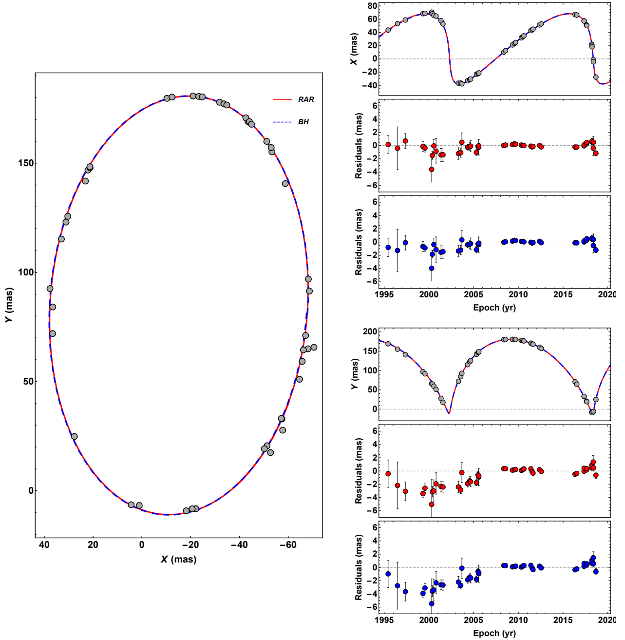
Fig. 2. Theoretical and observed orbit of S2 around Sgr A*. Left panel: orbit ( X vs. Y ), right panel: X and Y position as a function of time and the respective residuals of the best-fit for each model. The theoretical models are calculated by solving the equations of motion of a test particle in the gravitational field of (1) a Schwarzschild BH of 4.075 \times 10^6 M_{\odot} (dashed blue curves), and (2) the DM distribution obtained from the extended RAR model for 56 keV fermions (red curves). The mass of the quantum core in the RAR model is 3.5 \times 10^6 M_{\odot} . Table 1 shows the parameters of each model. We used the observational data reported in Do et al. (2019).
