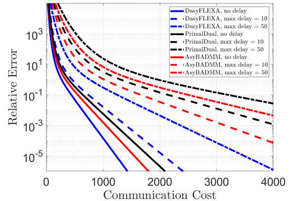
Fig. 2: LASSO problem: Relative error vs. # of message exchanges.
