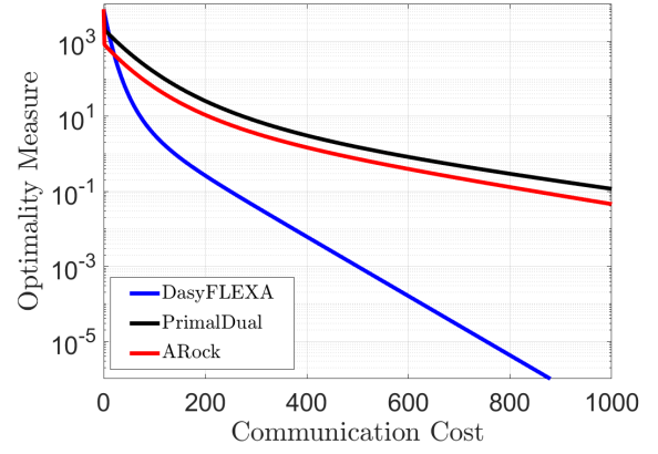
Fig. 4: Matrix completion: stationarity distance vs. # of message exchanges.
