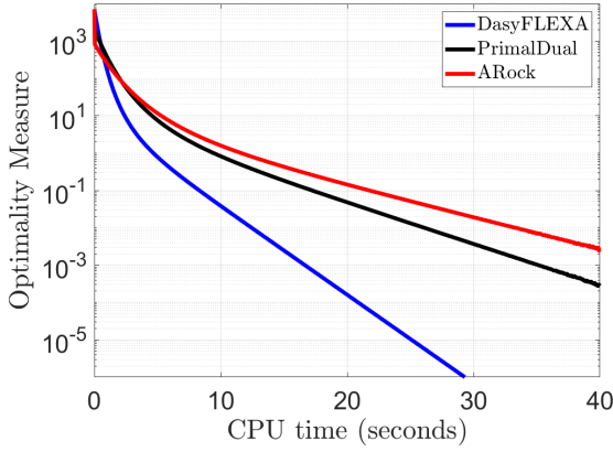
Fig. 3: Matrix completion: stationarity distance vs. # CPU time (in seconds).
