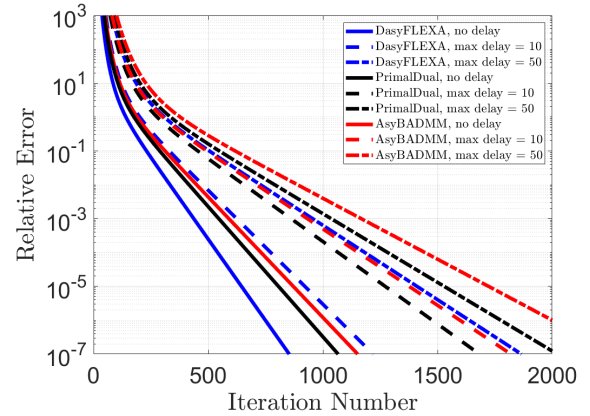
Fig. 1: LASSO problem: Relative error vs. # of iterations.
