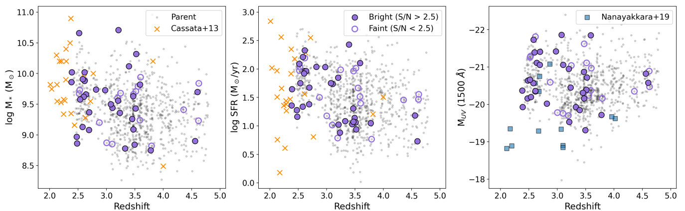
Fig. 5: Distribution of the derived stellar masses ( left ), star-formation rates ( centre ), and rest-frame UV magnitudes ( right ) of Bright (filled circles) and Faint (open circles) He II emitters with redshift. Also shown are measurements for the Parent sample (grey dots) and for He II emitters reported by Cassata et al. (2013) (orange crosses) and Nanayakkara et al. (2019) (blue squares). For our sample, we do not see any significant differences between the stellar masses, SFRs, and UV magnitudes of He II emitters and the parent sample. Our measurements are also comparable with those from the literature, although the Cassata et al. (2013) sample probes lower redshifts compared to both the Nanayakkara et al. (2019) and our He II emitters.
