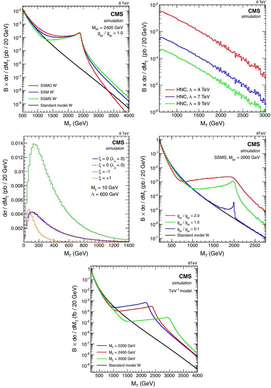
FIG. 3 (color online). Signal shapes at generator level: SSM model compared to the SSMS and SSMO models for g_{W^+}/g_{W^-} = 1 (top left), HNC-CI model for various values of \Lambda (top right), DM for various values of \xi (middle left), W' with W -boson interference and a varying coupling strength g_{W^+}/g_{W^-} in the same sign scenario (middle right), and \text{TeV}^{-1} model (bottom).
