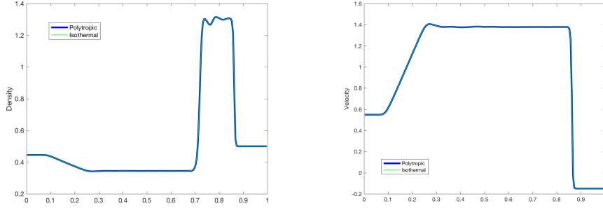
FIG. 5.6. Solutions at t_{\max} = 0.15 for initial data (5.5), using the fifth order well-balanced schemes for g = 1 .
