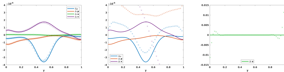
FIG. 5.12. Perturbation of a windy equilibrium at t = 0.4 . Vertical cut of the solution. Solid lines: reference solution (following the legend, perturbations in density, pressure, horizontal and vertical velocities, respectively). Left: Fully WB (circles) on a coarse grid; middle: Semi WB (crosses) for density, pressure and vertical velocity; right: Semi WB (crosses) for the horizontal velocity.
