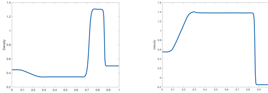
FIG. 5.5. Solutions at t_{\max} = 0.15 for initial data (5.5), using the third order well-balanced schemes for g = 1 .
