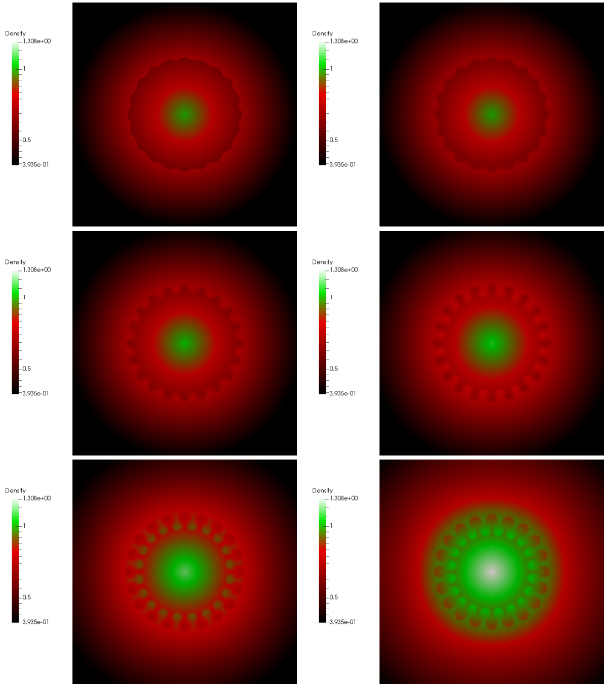
FIG. 5.9. Third order well balanced scheme on 400 \times 400 grid: times 0 to 4.0 equispaced
