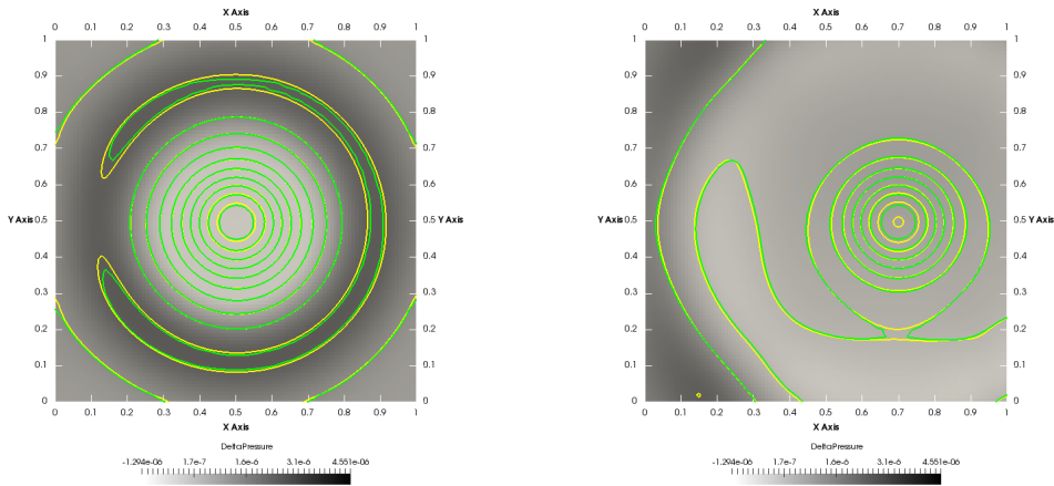
FIG. 5.10. Perturbation of a windy equilibrium: t = 0.2 on the left, and t = 0.4 on the right. Contours of the density fluctuations: reference solution (yellow), and Fully WB (green).
