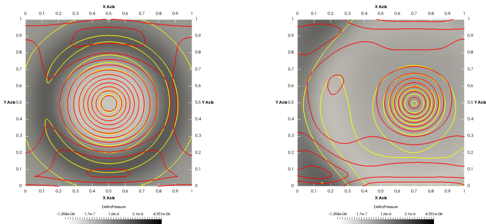
FIG. 5.11. Perturbation of a windy equilibrium: t = 0.2 on the left, and t = 0.4 on the right. Contours of the density fluctuations: reference solution (yellow), and Semi WB (red).
