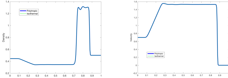
FIG. 5.7. Solutions at t_{\max} = 0.15 for initial data (5.5), using the fifth well-balanced schemes for g = 0 .
