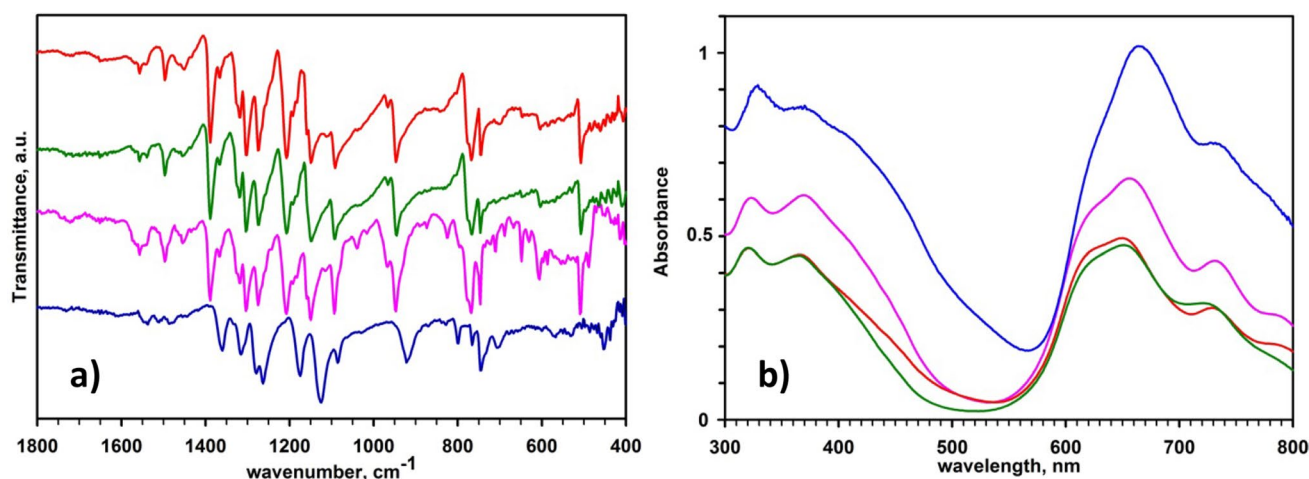
Fig. 1 a Infrared spectra and b UV–vis spectra of PG36 (blue solid line), PG7 (pink solid line), D-GC (green solid line) and E-GC (red solid line). The infrared spectra are taken on powder pigments or
