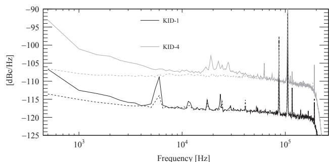
Fig. 2. Average noise power spectra for amplitude (dotted line) and phase (continuous line) read-out of a typical high-Q (KID-4) and a low-Q (KID-1) resonators. The flat noise is consistent with the amplifier noise. At low frequency another source of noise, not yet identified, appears in the phase noise power spectra, spoiling the energy resolution.
