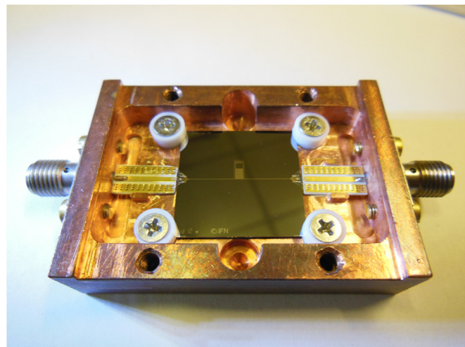
Fig. 1. A single Al KID deposited on a 2 × 2 cm 2 Si substrate. The chip was assembled in a copper structure using four PTFE elements.
