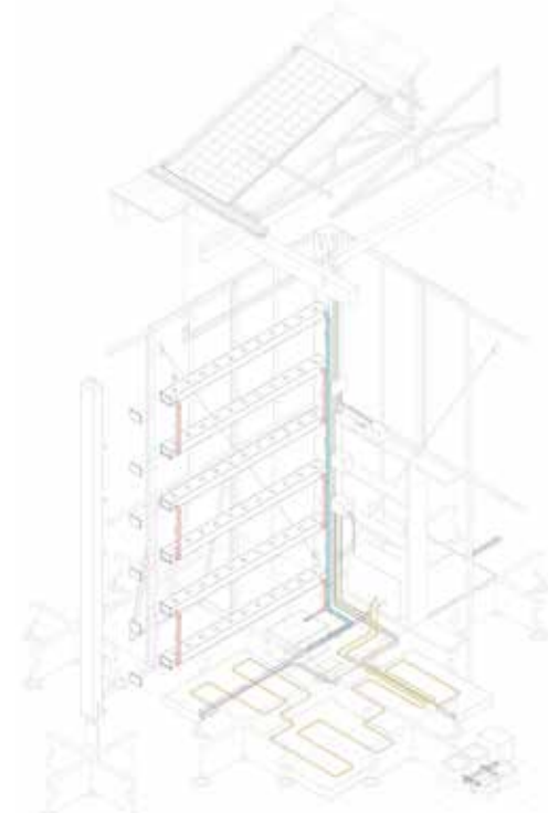
Intrinsic Circularity of the Greenhouse Mechanical and electrical systems axonometric cross section
