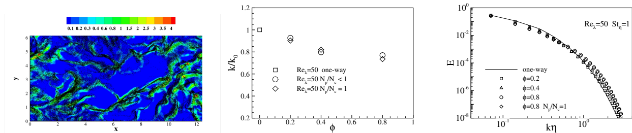
Figure 1. Left panel: snapshot of the instantaneous particle configuration (scatter plot) and of the ensuing Eulerian intensity of the force feedback field operated by the particles on the fluid (contour plot). The slice in the x - y is of the order of few Kolmogorov scales. The mean flow U(y) = Sy is in the x - y plane from left to right. Central panel: Normalized turbulent kinetic energy versus the mass loading \Phi . Data obtained for few particles per cell N_p/N_c < 1 are compared against data with N_p/N_c = 1 . Right panel: Energy spectrum at different values of the mass loading, namely \Phi = 0.2, 0.4, 0.8 and at different values of the number of particles per cell.
