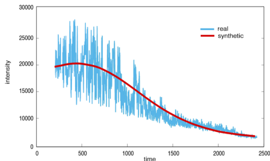
Figure 16: In red the synthetic lightcurve found by the algorithm. In blue the real lightcurve of the Tiangong-1 passing over Rome the 15/02/2018
