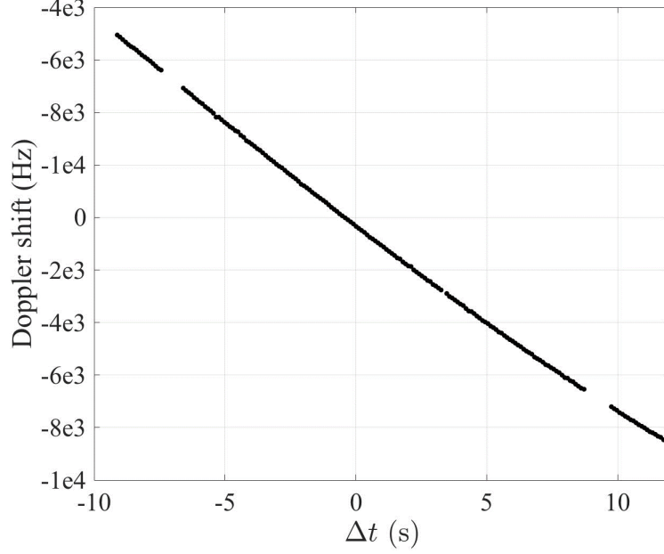
Figure 11: DS profile measured by BIRALES
