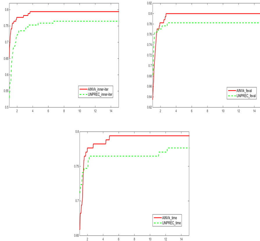
FIG. 2. Comparison between the unpreconditioned and preconditioned (AINVK) truncated Newton method, in terms of inner iterations (top left), number of function evaluations (top right) and CPU time (bottom)
