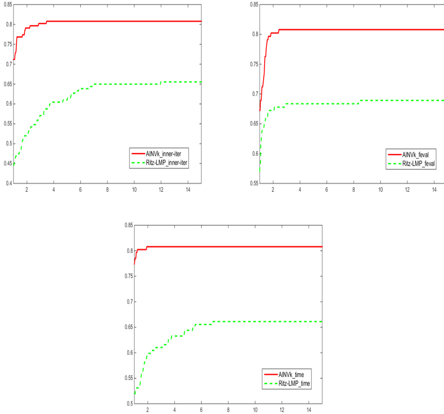
FIG. 3. Comparison between the AINVK and Ritz-LMP preconditioners on the whole set of test problems, in terms of inner iterations (top left), number of function evaluations (top right) and CPU time (bottom)
