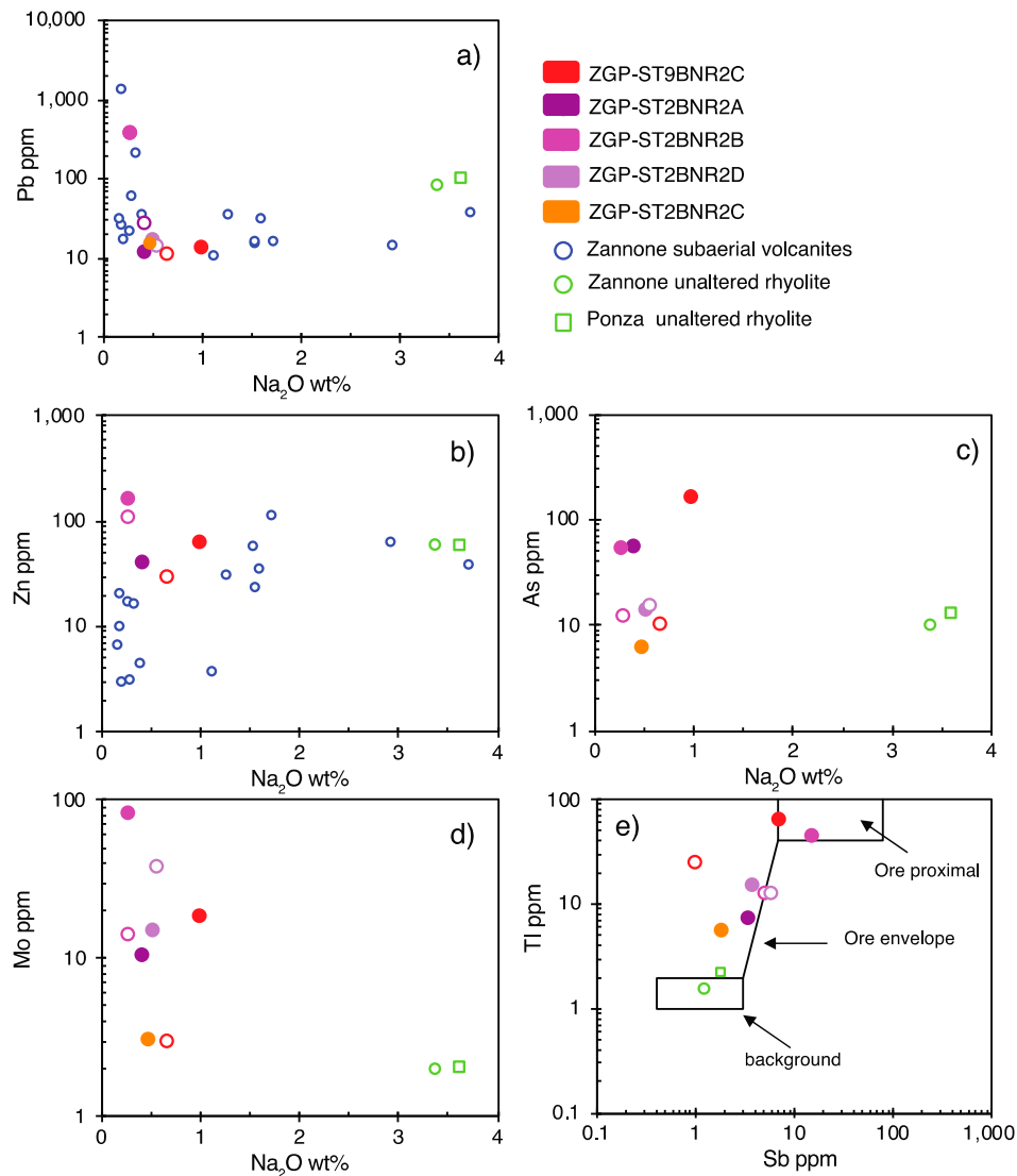
Figure 14. (a–d) Correlation plots of \text{Na}_2\text{O} against selected base metal elements and As. (e) Relationship between Sb and Tl diagram for differently hydrothermal altered ZGP rhyolite clasts. The fields are from Large et al. [22]. Here and in Figure 15, Zannone subaerial volcanites are from Conte and Dolfi [26]. Data of unaltered Zannone and Ponza volcanics are from Conte et al. [28]. Symbols of ZGP clasts: full—inner portion, empty—outer portion.
