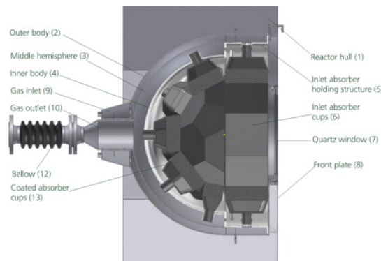
Figure 10. Sectional view of the spherical cavity reactor proposed by Houaijia et al. Reprinted from [4] with permission from Elsevier.
