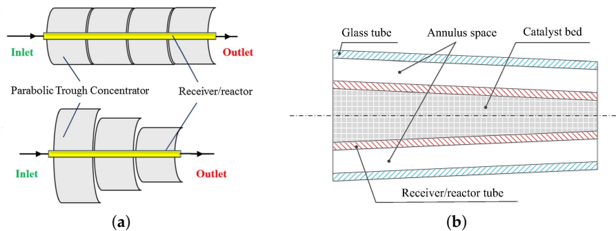
Figure 9. (a) Comparison between the traditional solar concentrator structure (top) and new solar concentrator structure (bottom); (b) reactor/receiver tube with variable diameter. Reprinted from [114] with permission from Elsevier.
