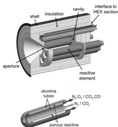
Figure 12. Indirectly heated solar reactor/receiver for water-splitting redox cycle on ceria (top) and detail of the reactive element. Reprinted from [119] with permission from ASME.
