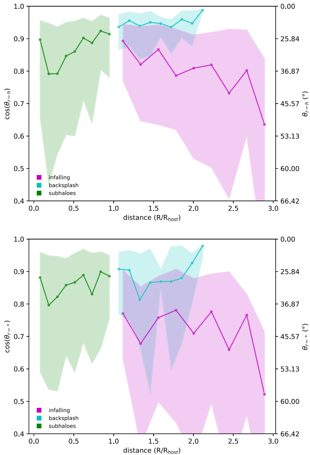
Figure 6. Median radial alignment – as defined by equation (4) using 25/75 percentiles as the error bars – of dark matter (upper panel) and stellar (lower panel) objects as a function of distance to the central galaxy cluster.
