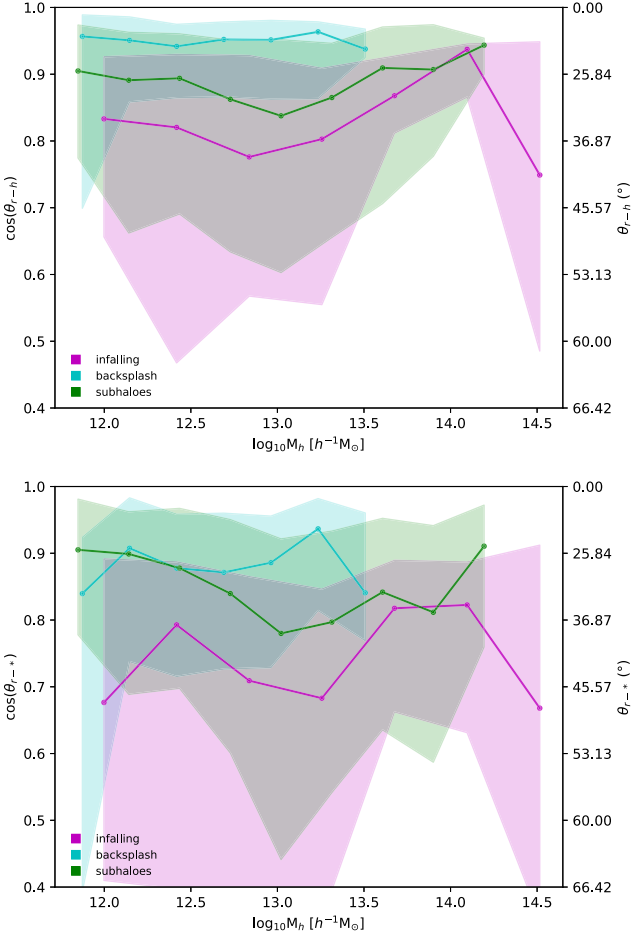
Figure 7. Median radial alignment of the dark matter ( \theta_{r-h} ; upper panel) and stellar ( \theta_{r-*} ; lower panel) component of objects as a function of their halo mass (error regions are again 25/75 percentiles).
