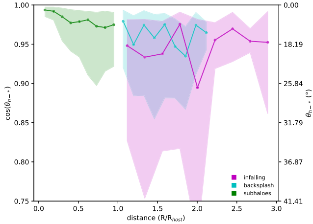
Figure 4. Median alignment between halo and stellar component as a function of distance to the (host) galaxy cluster; errors are again 25/75 percentiles. Values closer to unity are representative of a stronger alignment.
