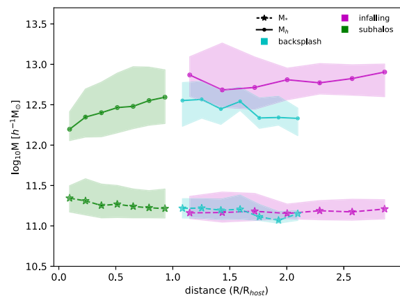
Figure A2. Median halo mass as a function of normalized distance to the host.
