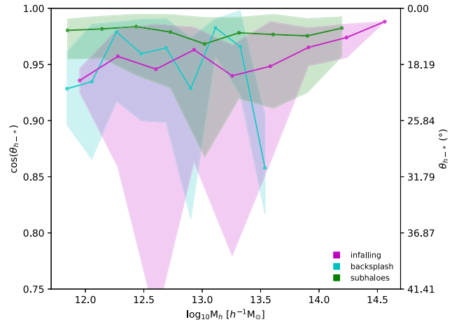
Figure 5. Alignment between halo and stellar component as a function of halo mass. Values closer to unity are representative of a stronger alignment.
