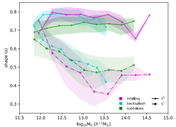
Figure 3. Halo and stellar component sphericities as a function of halo mass. In this and all subsequent plots, the values shown are the median in the respective bin with the error bars representing 25/75 percentiles.
