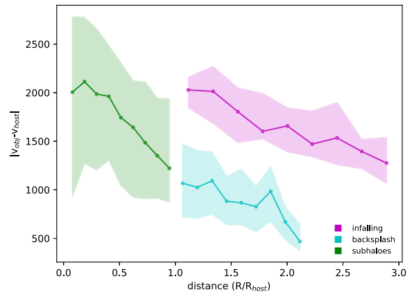
Figure A3. Halo velocity in host rest frame as a function of distance to the host.
