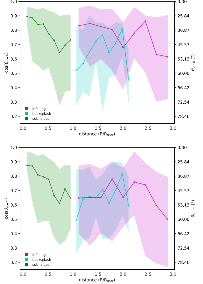
Figure 8. Alignment of the halo (upper panel) and stellar (lower panel) component with the bulk velocity vector of the halo in the rest frame of the central galaxy cluster. Values closer to unity are representative of the object’s major axis \mathbf{e}_a being aligned with the direction in which the object is moving.
