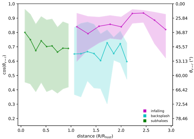
Figure 9. Alignment between the bulk velocity vector and the radial position vector of the haloes in the rest frame of the central galaxy cluster. Values closer to unity are representative of a stronger alignment.
