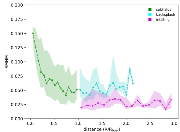
Figure A1. SMHM ratio as a function of normalized distance to the host.
