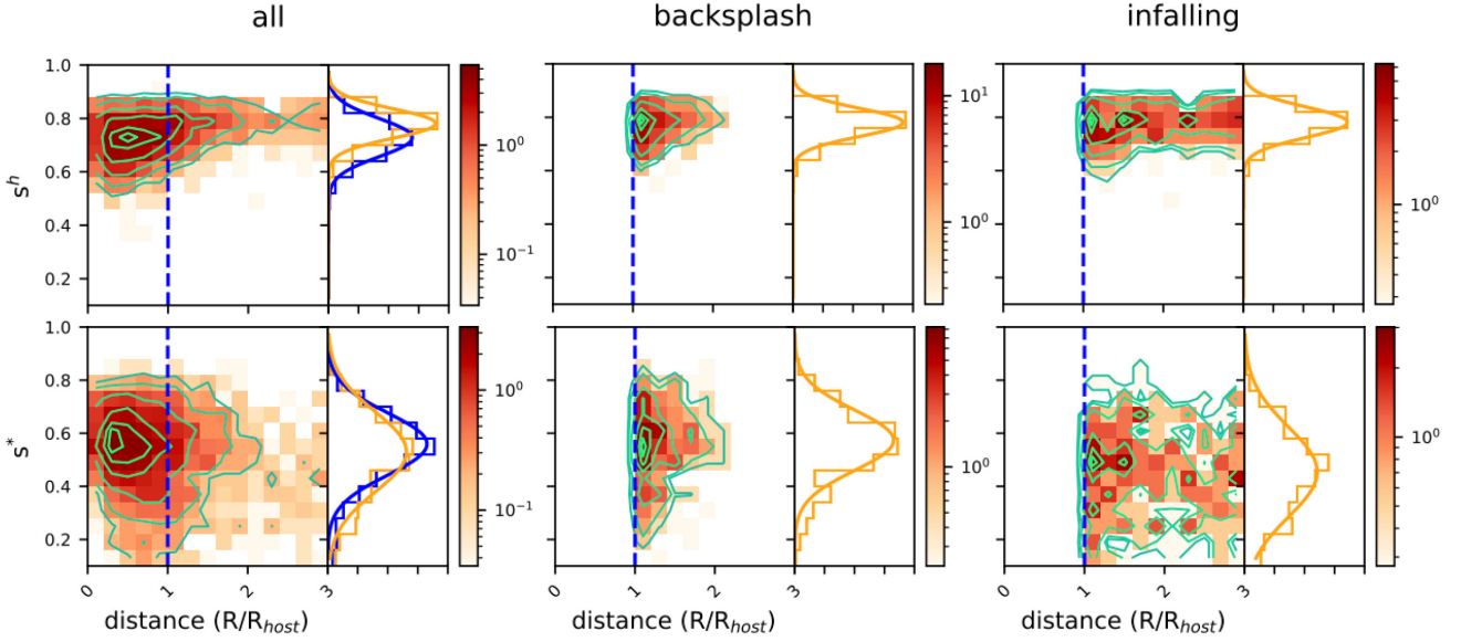
Figure 2. Halo (upper panel) and stellar component (lower panel) sphericities as a function of distance to the centre of the (host) galaxy cluster. The panels to the right of each contour plot show the respective distribution of sphericities for objects inside (blue) and outside (orange) R_{\text{host}} = R_{200c} of the central host cluster. The vertical blue-dashed line corresponds to R_{200c} . While we use all objects in the left-hand panel, the data are restricted to backsplash (infalling) objects in the middle (rightmost) one. The colour bar encodes the number of objects in each bin.
