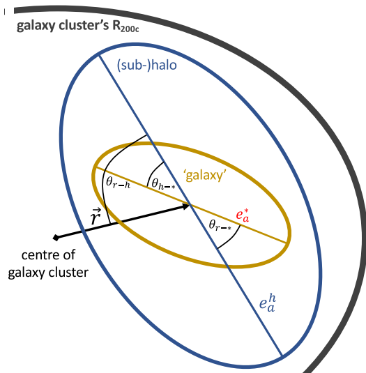
Figure 1. Illustration of the eigenvectors and angles used for the study of alignments.
