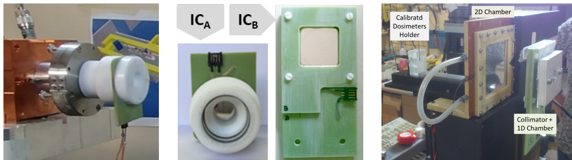
Figure 3. Left: the IC_A in place at the beam pipe exit. Middle: the two integral chambers, IC_A with its cylindrical holder acts as a plug on the beam pipe terminal and the IC_B . Right: the typical configuration during calibration and irradiation: IC_B with an aluminum collimator, in front of the 2D-IC; beyond them the holder of the calibrated dosimeters (e.g. microDiamond, alanine pallets and other devices).
