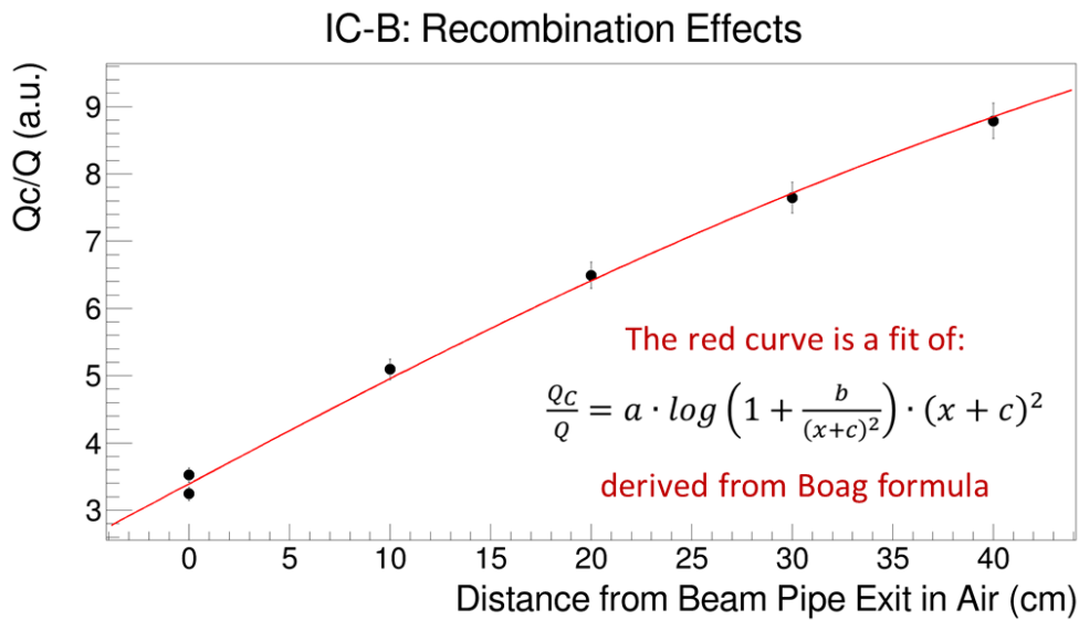
Figure 8. Recombination effects in the integral chamber IC_B : ratio of the collected Q_c and produced Q charges in the chamber versus the beam pipe exit window distance in air (and therefore the beam transverse size). The fitting curve is described in the text, \chi_r^2 = 1.64 .
