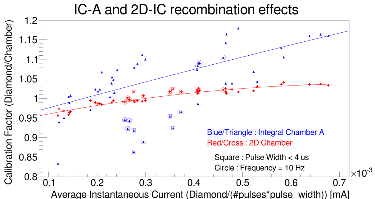
Figure 5. Evidence of recombination effects in \text{IC}_A and 2D-IC; dose rate variation induced by current, width, frequency of the pulses; the typical therapeutic dose rate of 1 Gy/min corresponds to about 0.2 mA on the x -axis.
