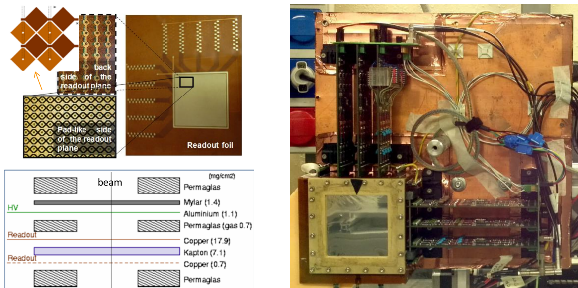
Figure 2. The 2D-IC chamber prototype. Left: pictures of its internal structure and a simplified drawing showing the peculiar pad-like strips pattern of the readout foil (above) and the cross section of the chamber (below). Right: picture of the assembled chamber with the dedicated discrete readout electronics of 48 \times and 48 \times y strips; a grounded cover (not shown) shields the whole electronics.
