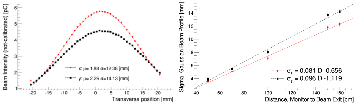
Figure 4. 2D-IC chamber response; left: x/y beam profiles measured at 160 \text{ cm}^2 from beam pipe exit, with Gaussian fits and relative parameters. Right: the widths measured by the 2D-IC profiles gaussian fits (sigma) at different distances from the beam pipe exit.
