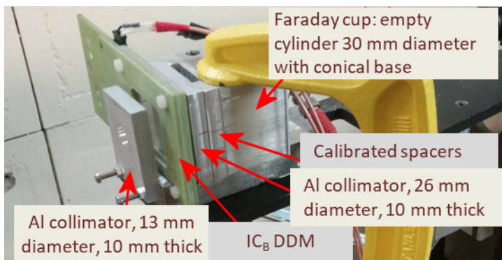
Figure 6. IC_B and FC assembly for recombination studies in the integral chamber.
