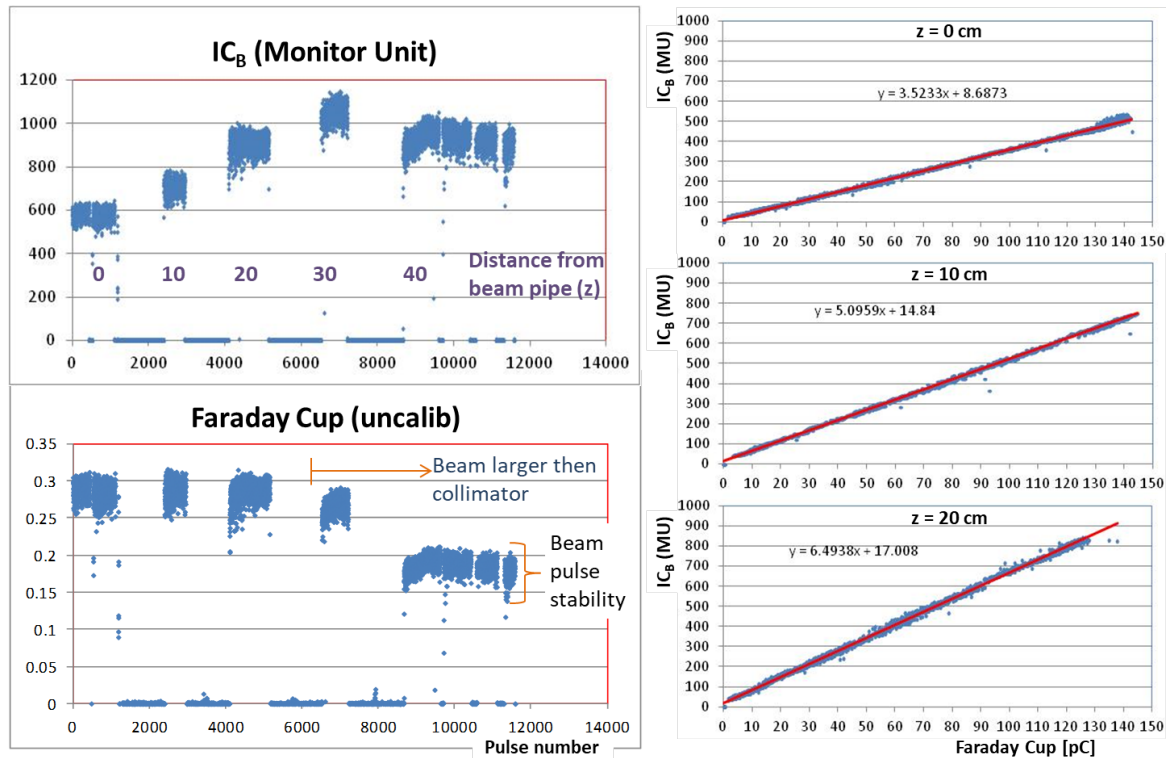
Figure 7. IC B and FC responses. Left: the two devices pulse-by-pulse responses at different distance from the beam pipe exit. Right: the response correlations for different dose rate (pulse intensities) and at different distances; in red the linear fits.
