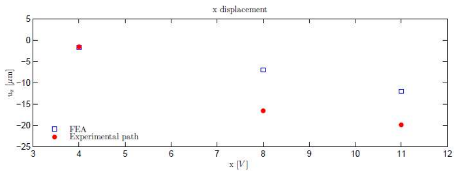
Figure 10. Comparison of the displacements obtained by the FEA model (blue squares) and the experimental measurements (red plain circles).
