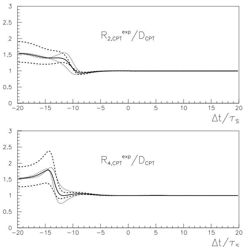
Figure 3. The expected ratios for the CPT test R_{2,CPT}^{exp}(\Delta t) (top) and R_{4,CPT}^{exp}(\Delta t) (bottom) as a function of \Delta t (solid line); dashed lines correspond to \pm 10\% variation in the absolute value of \eta_{3\pi^0} , while dotted lines correspond to a \pm 10^\circ variation of its phase (with respect to the value \eta_{3\pi^0} = \epsilon_S ). For visualization purposes the CPT violating parameters have been fixed to the values \Re\delta = 3.3 \times 10^{-4} and \Im\delta = 1.6 \times 10^{-5} .
