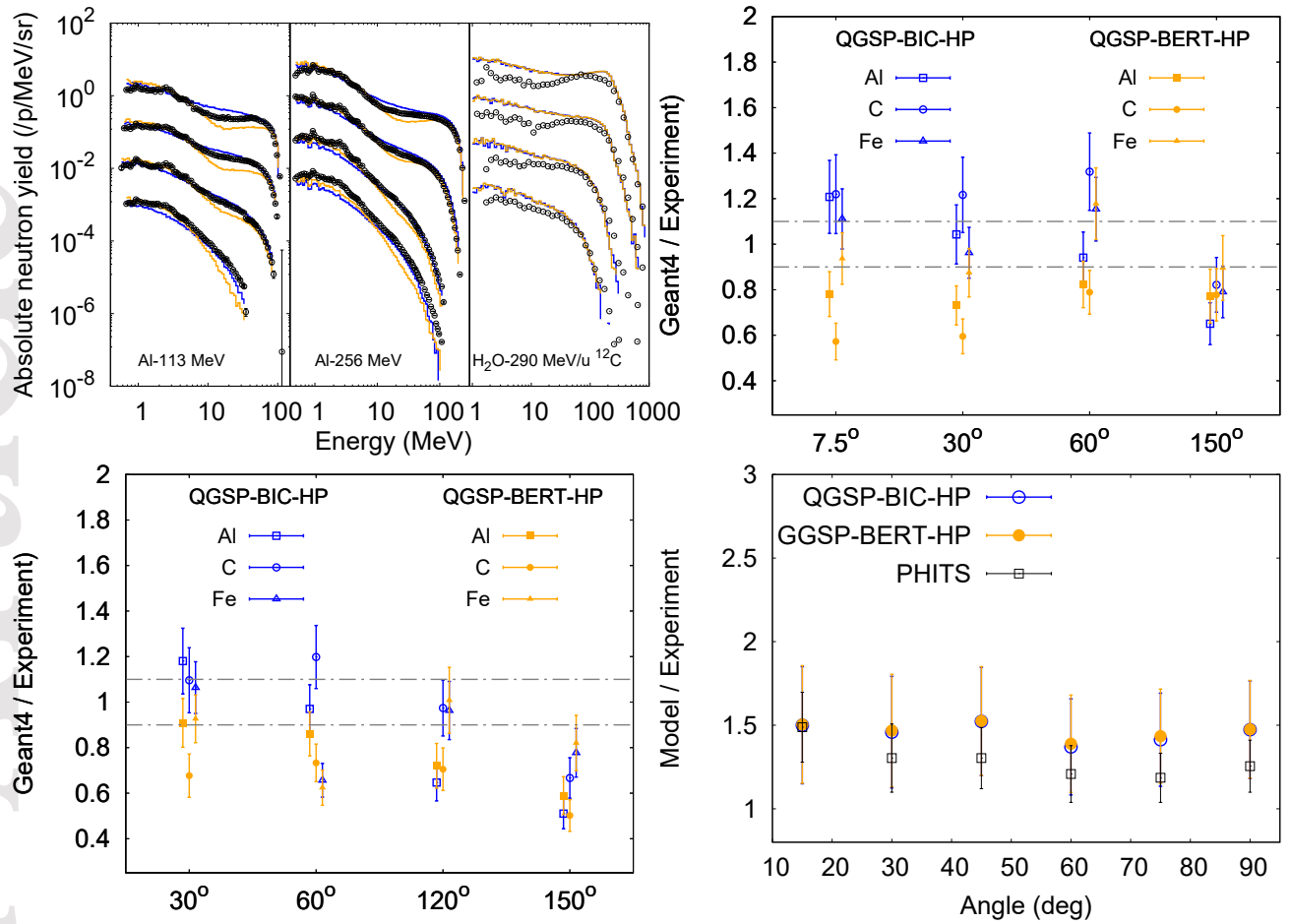
FIG. 18. Absolute neutron yield (top left) for protons of 113 MeV and 256 MeV impinging an aluminum target and 290 MeV/u carbon ions in a water phantom. Geant4 calculation using QGSP_BIC_HP is shown with blue solid line whereas results with QGSP_BERT_HP is shown with orange solid lines. Experimental data are shown with empty markers. Ratio between calculated to experimental integrated neutron yield for 113 MeV protons (top right), 256 MeV protons (bottom left) and 290 MeV/u carbon ions (bottom right). The gray dashed line represents the experimental uncertainty, one standard deviation ( \sigma_{ref} ). Error bars represent one standard deviation.
