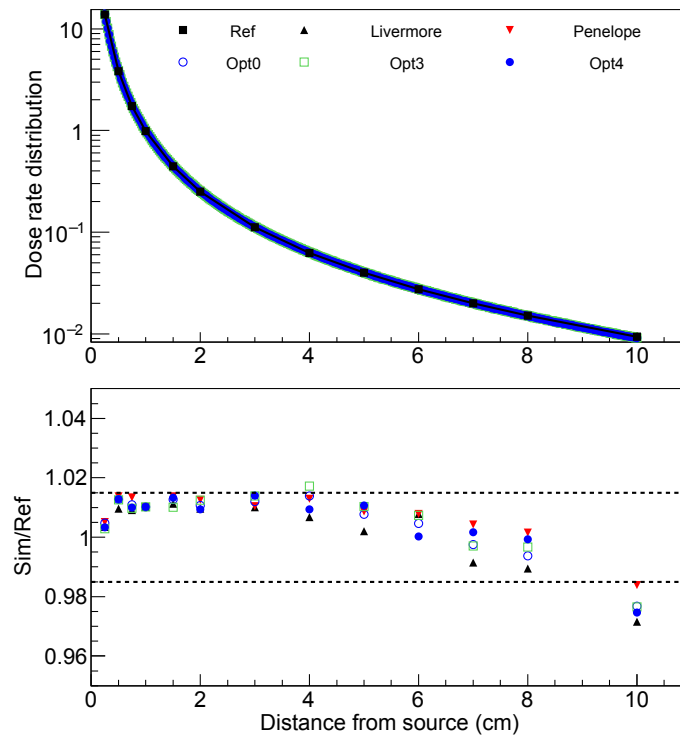
FIG. 11. Radial dose rate distribution with respect to r , distance from the center of the ^{192}\text{Ir} brachytherapy source. The radial dose distribution is normalised at r=1 cm. Black squares in the top figure represent the reference data (from Granero et al 2006 [83]), the statistical uncertainties of the data are within the symbols. The bottom plot shows the ratio of the Geant4 simulation results and the reference data. The dashed lines indicate the statistical uncertainty affecting both the simulation results obtained with Geant4 10.5 and the reference data published in Granero et al 2006 [83], obtained with Geant4 7.1.
