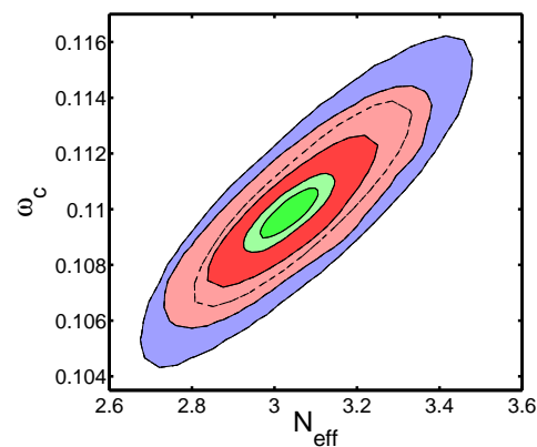
Figure 5. 68% and 95% likelihood contour plots on the N_{eff} - \omega_c plane for Planck (blue), Planck+ACTPol (red) and CMBPol (green).
