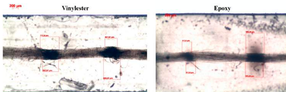
Figure 7. Typical optical micrographs of fragmented flax yarns in vinylester and epoxy matrices: measurement of the debonding length ( l_{\text{debonding}} ).
