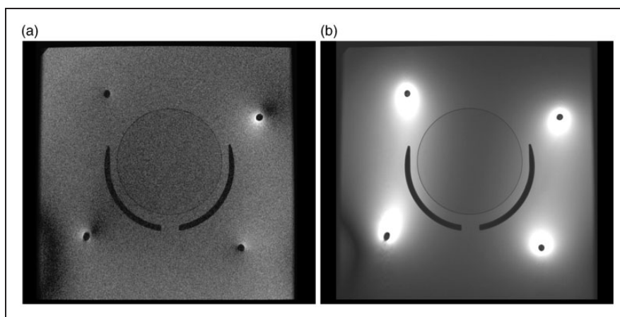
Figure 4. Example of the magnetic resonance imaging (MRI) scans used for signal-to-noise ratio measurements at 1.5T using a daily quality assurance gel phantom set-up. Axial scans acquired with the MRI body radiofrequency coil (a) and with the dedicated two-channel FUS-Head coil (b). Scan parameters reported in Table 1; images from acquisitions with four averages are shown.
