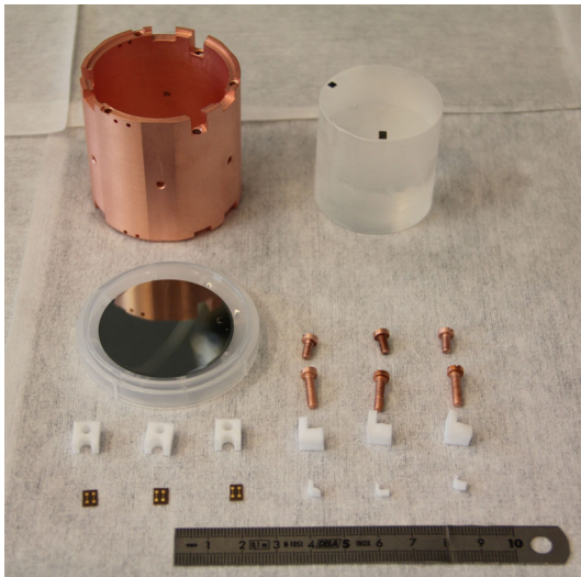
Fig. 3 All components used to assemble a CUPID-Mo single detector module: a copper holder, a Li 2 100 MoO 4 crystal with glued NTD and heater, a Ge LD with NTD, the copper screws, the PTFE spacers and fixing elements, the Kapton foil with golden pads. Note that the reflecting film is not shown here
