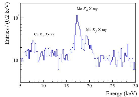
Fig. 9 Energy spectrum of CUPID-Mo light detector LD2 after a 33 h ^{60}\text{Co} irradiation in the EDELWEISS-III set-up. The Mo K_{\alpha} X-rays are used for the LD calibration
