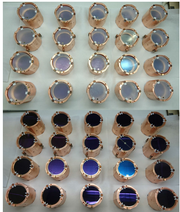
Fig. 5 Twenty CUPID-Mo detector modules before their arrangement in five towers; the devices are shown from the Li 2 100 MoO 4 crystal side (top) and from the Ge LD side (bottom)
