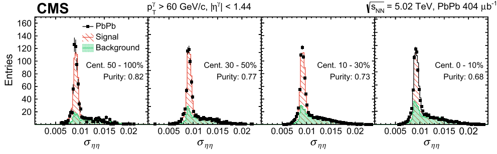
Fig. 1. The centrality dependence of the shower shape variable \sigma_{\eta\eta} for photons with p_T^\gamma > 60 GeV/c. The black points show the PbPb experimental results, the red histograms are the signal templates from PYTHIA+HYDJET simulations, and the green histograms are the background templates obtained from a nonisolated sideband region in data. (For interpretation of the colors in the figure(s), the reader is referred to the web version of this article.)
