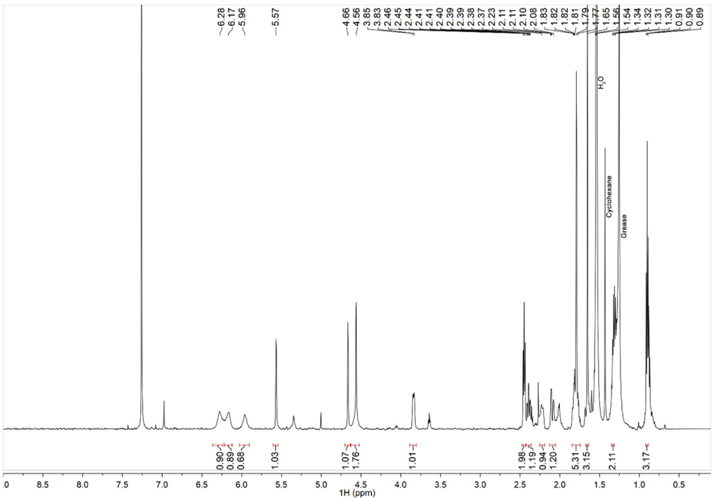
Fig. 7. ^1\text{H-NMR} of isolated CBD.
