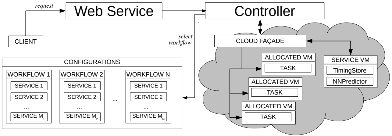
Fig. 1. The overall configuration of the developed system.
