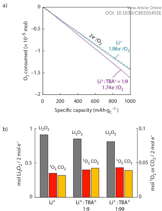
Fig. 3 Superoxide disproportionation and ^1\text{O}_2 formation during \text{Li-O}_2 cell discharge. (a) \text{O}_2 consumption vs. capacity upon discharge of carbon black electrodes at a rate of 100 \text{ mA}\cdot\text{g}_c^{-1} in \text{O}_2 saturated TEGDME electrolytes that contained 30 mM DMA and either 0.1 M \text{Li}^+ or a total of 1 M salt with a \text{Li}^+:\text{TBA}^+ ratio of 1:9 or 1:99. The 1:99 ratio is given in Fig. S9 and voltage profiles in Fig. S10. (b) Obtained \text{Li}_2\text{O}_2 , ^1\text{O}_2 , and \text{Li}_2\text{CO}_3 (expressed as \text{CO}_2 ) per 2 e^- passed in the cells shown in (a).
