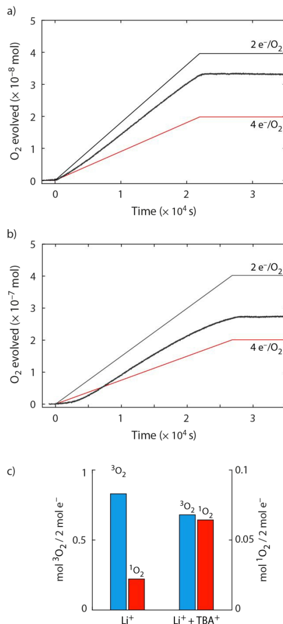
Fig. 4 Superoxide disproportionation and ^3\text{O}_2 formation during \text{Li}-\text{O}_2 cell charge. (a,b) \text{O}_2 evolution vs. time upon charge of carbon black/ \text{Li}_2\text{O}_2 /PTFE (9/1/1, m/m) composite electrodes in TEGDME electrolyte containing 30 mM DMA and 0.1 M \text{Li}^+ (a) or 0.1 M \text{Li}^+ and 0.9 M \text{TBA}^+ (b). Electrodes were charged at a rate of 10 \text{ mA}\cdot\text{g}_c^{-1} until 3.95 V and then kept at open circuit until the pressure was stable. (c) ^3\text{O}_2 and ^1\text{O}_2 obtained per 2 e^- passed for the cells shown in (a) and (b).
