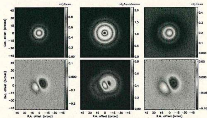
Figure 8. Application of the filters to point source residuals in case 1 (no source subtraction, top) and case 2 (source improperly subtracted, bottom). The input point source flux has been normalized to one. Left: input surface brightness map. Middle: GGM filtered map. Right: DoG filtered map.
