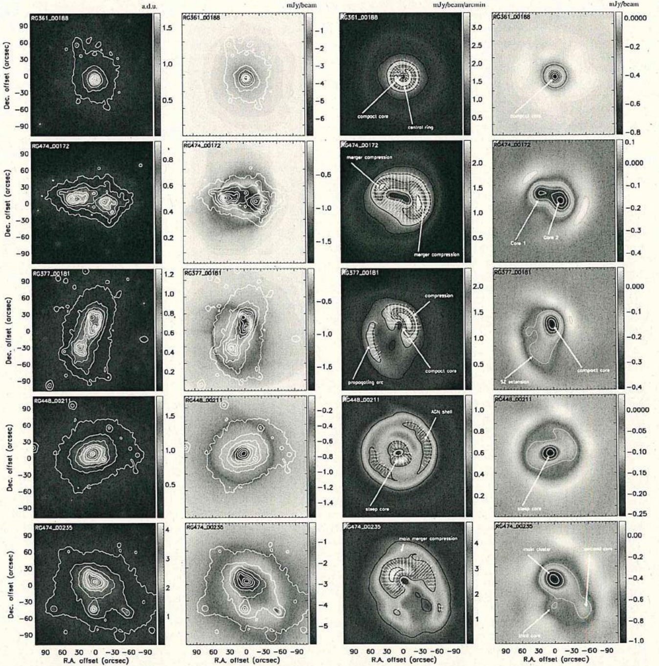
Figure 4. Application of the filtering algorithms to clusters from the RHAPSODY-G suite of simulations. From top to bottom, the clusters are RG361_00188, RG474_00172, RG377_00181, RG448_00211, and RG474_00235 (see also Table 2 for the main properties of the sample). Left: projected dark matter density. Contours are linearly spaced. Units are arbitrary. Middle left: input raw tSZ surface brightness maps with dark matter map contours overlaid. Units are mJy/beam. Middle right: GGM filtered maps with \theta_0 = 15'' . The white vectors represent the direction of the gradient, \Psi . Units are mJy/beam/arcmin. Right: DoG filtered maps with \theta_1 = 15'' and \theta_2 = 45'' . Units are mJy/beam. The contours provide the true signal-to-noise expected for the simulation of the observation of these sources done in Section 5. They are given by steps of 2\sigma excluding 0 (see Section 5 for further discussions about the signal-to-noise estimates).
