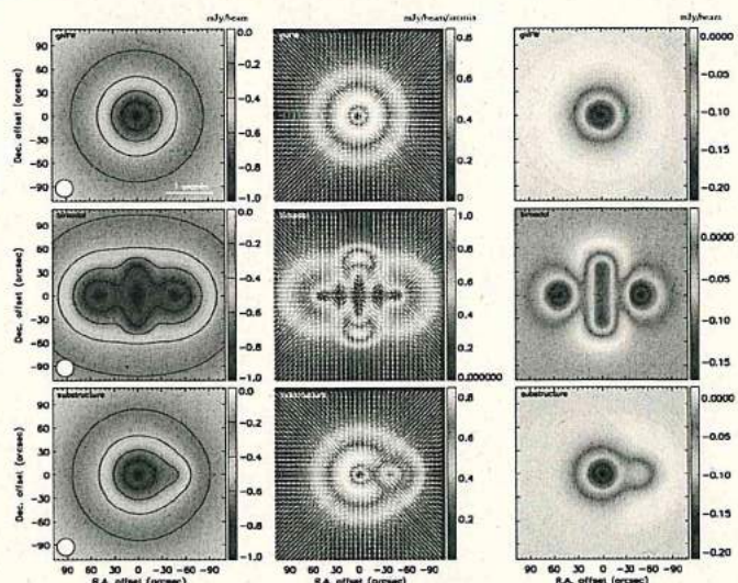
Figure 2. Surface brightness and GGM and DoG response to the tSZ signal expected for a spherically symmetric gNFW pressure profile (top), a bimodal cluster plus a pressure bar (middle), and a main core plus an extension (bottom). Left: tSZ simulated surface brightness. The white circle on the bottom left provides the beam FWHM. Middle: GGM filtered maps with \theta_0 = 15'' . The white vectors represent the direction of the gradient, \Psi . Right: DoG filtered maps with \theta_1 = 15'' and \theta_2 = 45'' .
