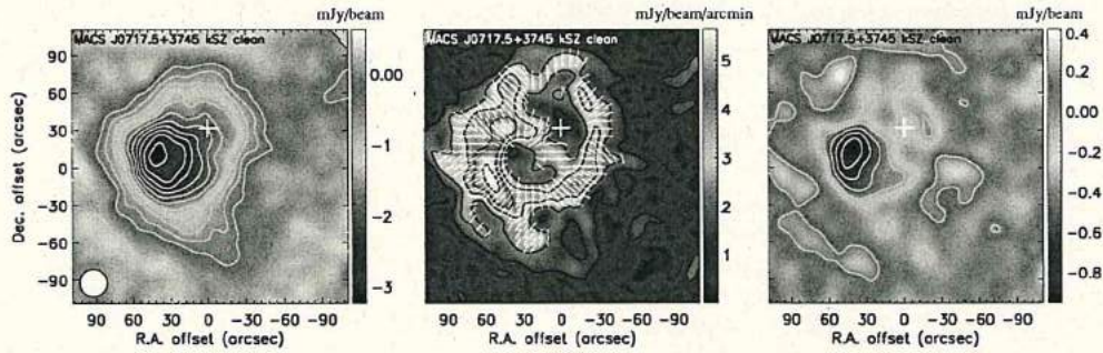
Figure C.1. Surface brightness (left), GGM (middle) and DoG (right) maps of MACS J0717.5+3745 in the case of kSZ correction applied. See figure 9 for further details.
