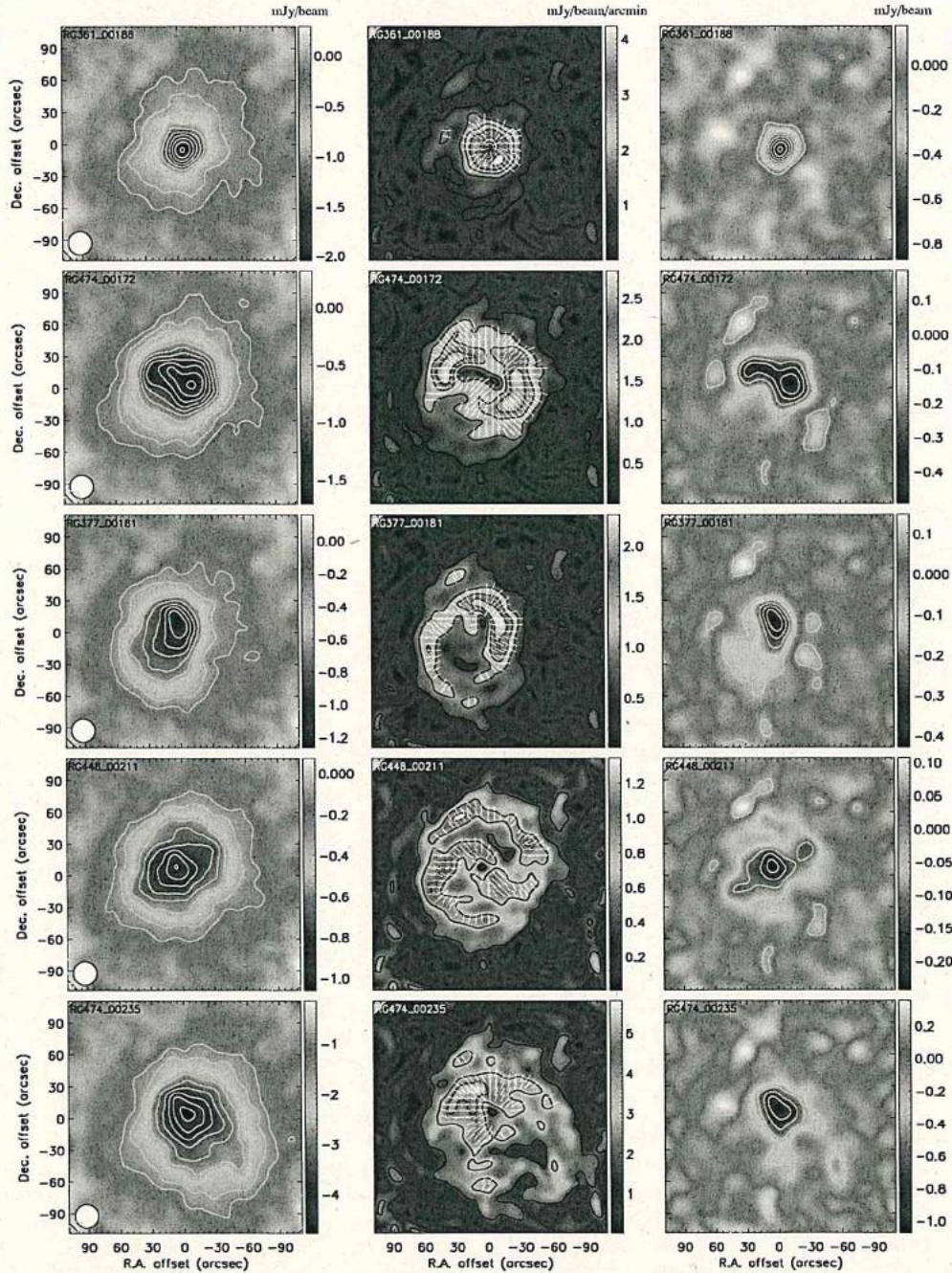
Figure 5. Same as figure 4 in the case of end-to-end processing of the simulated RHAPSODY-G sub-sample: surface brightness maps (left), GGM filtered maps (middle) and DoG filtered maps (right). From top to bottom, the clusters are RG361_00188, RG474_00172, RG377_00181 and RG448_00211 (see also Table 2 for the main properties of the sample). The surface brightness images are deconvolved from the transfer function (but not from the beam smoothing) and the signal-to-noise contours are estimated as in the case of real data (separated by steps of 2\sigma ).
