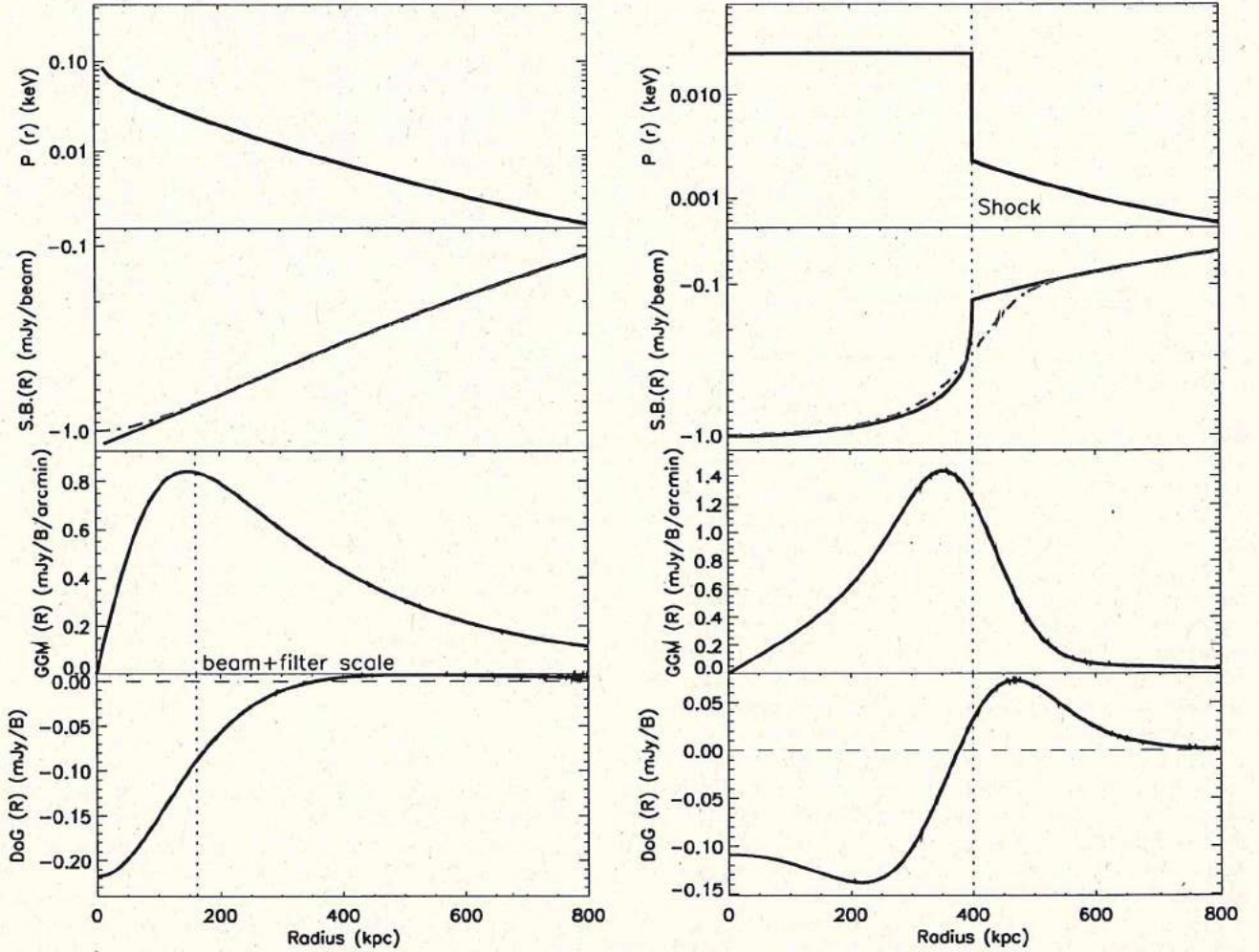
Figure 3. Left: GGM and DoG response to a gNFW radial pressure profile. The vertical dashed line provide the physical size corresponding to the 15 arcsec filter plus the NIKA beam size, at the cluster redshift. Right: GGM and DoG response to a shock propagating outward, in a radially symmetrical way, with Mach number \mathcal{M} = 3 . The shock position is given by the vertical dashed line. From top to bottom, we show the pressure, the surface brightness, the GGM and the DoG radial profile. In the surface brightness case, the thick black lines provide the raw profile while the thin red dashed-line accounts for beam smoothing. The pressure depends of the physical radius in 3D, while the other quantities depend on the projected radius, in 2D.
