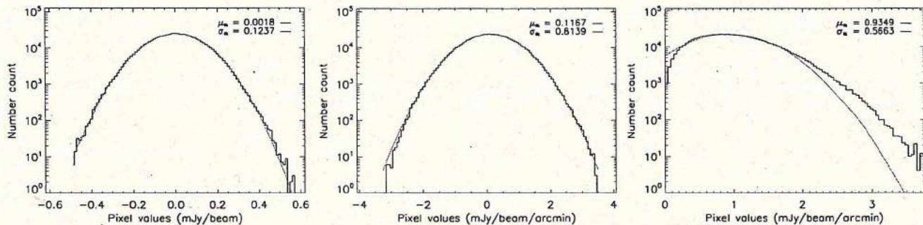
Figure 6. Noise distribution of all the pixels enclosed within 30 arcsec radius from the cluster center, in the case of CL J1226.9+3332, for our baseline filter parameters. The red curves provides the best Gaussian fit to the histograms. Left: DoG noise histogram. Middle: GGM noise histogram in the case of \hat{\delta} set to the observed signal of CL J1226.9+3332. Right: GGM noise histogram in the case where \hat{\delta} = 0 in Eq 8.
