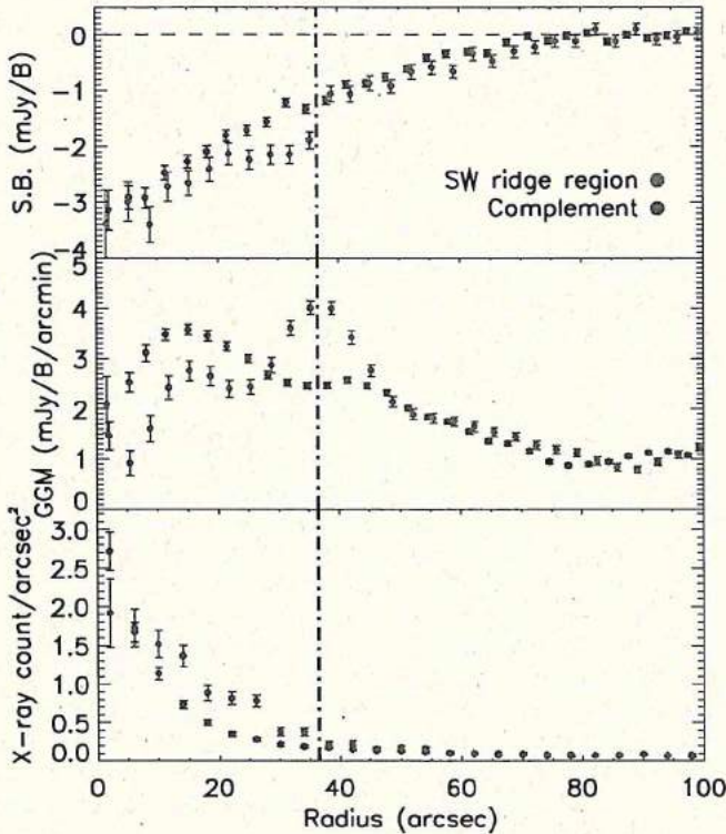
Figure 12. Comparison of the profile of CL J1226.9+3332 in the region of the GGM ridge (green) to its complement (red). The GGM ridge region is define in Figure 9, as the black dashed line on the surface brightness image. The dashed-dotted line correspond to the GGM ridge location. Top: surface brightness profile. Middle: GGM profile. Bottom: Chandra photon count per unit area profile.
