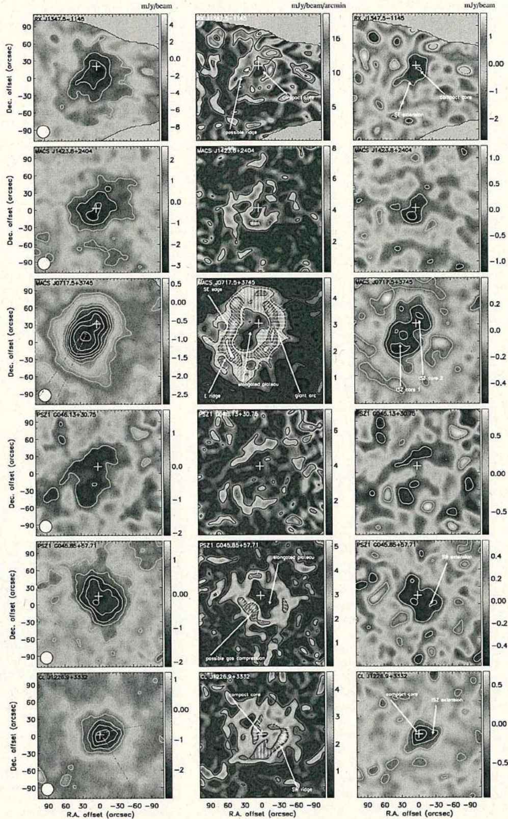
Figure 9. Redshift-ordered maps of the NIKA cluster sample at 150 GHz. Left: Surface brightness images. Each map has been smoothed to an effective angular resolution of 22 arcsec FWHM, as shown by the bottom left white circle. Point sources have been subtracted and the data have been deconvolved from the transfer function, but the zero level absolute brightness remains unconstrained. Middle: GGM filtered maps. Right: DoG filtered maps. In all cases, contours provide the signal-to-noise ratio, starting at \pm 2\sigma and increasing by 2\sigma steps. The white crosses provide the main X-ray peak (see Table 3). In the case of MACS J0717.5+3745, the kSZ contribution is not accounted for in the map presented here (see Appendix C and Section 6.3 for more details). In the case of CL J1226.9+3332 and MACS J0717.5+3745, the dashed lines correspond to the cone used to define the GGM ridge region when extracting profiles in Figure 12 and 11.
