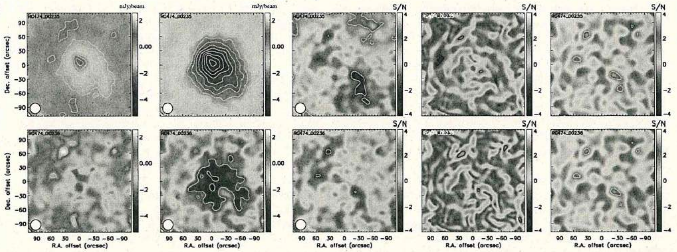
Figure B.1. Effect of the deconvolution on the processed map (first two columns) and difference between the expected signal and the recovered signal (3 last columns), in the case of the very massive and nearby test cluster RG474.00235. The top panel correspond to the high signal-to-noise case, and the bottom panel to the low signal-to-noise case, with a peak signal-to-noise of about 20 and 3, respectively, at the 22 arcsec resolution. From left to right, we provide: the raw processed surface brightness, the deconvolved surface brightness, the deconvolved surface brightness difference map, the GGM difference map, and the DoG difference map. In all cases, contours provide the signal-to-noise ratio, starting at \pm 2\sigma and increasing by 2\sigma steps.
