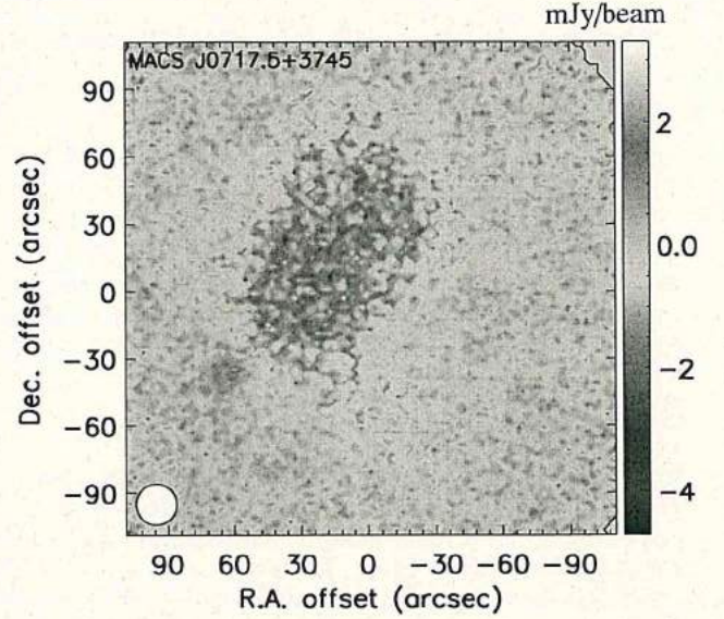
Figure 1. Example of the raw surface brightness image of MACS J0717.5+3745, prior to any filter application (e.g. smoothing), point source removal and deconvolution. The data is dominated by noise on small scales. The cluster diffuse emission is nonetheless visible as a negative decrement, as well as a radio foreground galaxy (positive) on the southeast. The white circle on the bottom left corner provide the NIKA beam FWHM.
