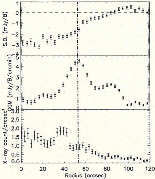
Figure 11. Profile of MACS J0717.5+3745 in the region defined to include the strongest GGM ridge (east ridge, see Figure 9, as the dark gray dashed line on the surface brightness image). The dashed-dotted line correspond to the GGM ridge location. Top: surface brightness profile. Middle: GGM profile. Bottom: Chandra photon count per unit area profile.
