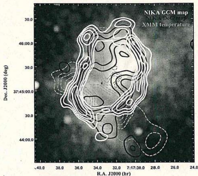
Figure 10. Multi-probe view of the cluster MACS J0717.5+3745: Chandra X-ray surface brightness image (ObsID4200), plotted on a square root scale (thus proportional to the projected density) with XMM-Newton temperature (green contours from Adam et al. 2017b) and the DoG (black contours) and GGM (white contours) maps overlaid.
