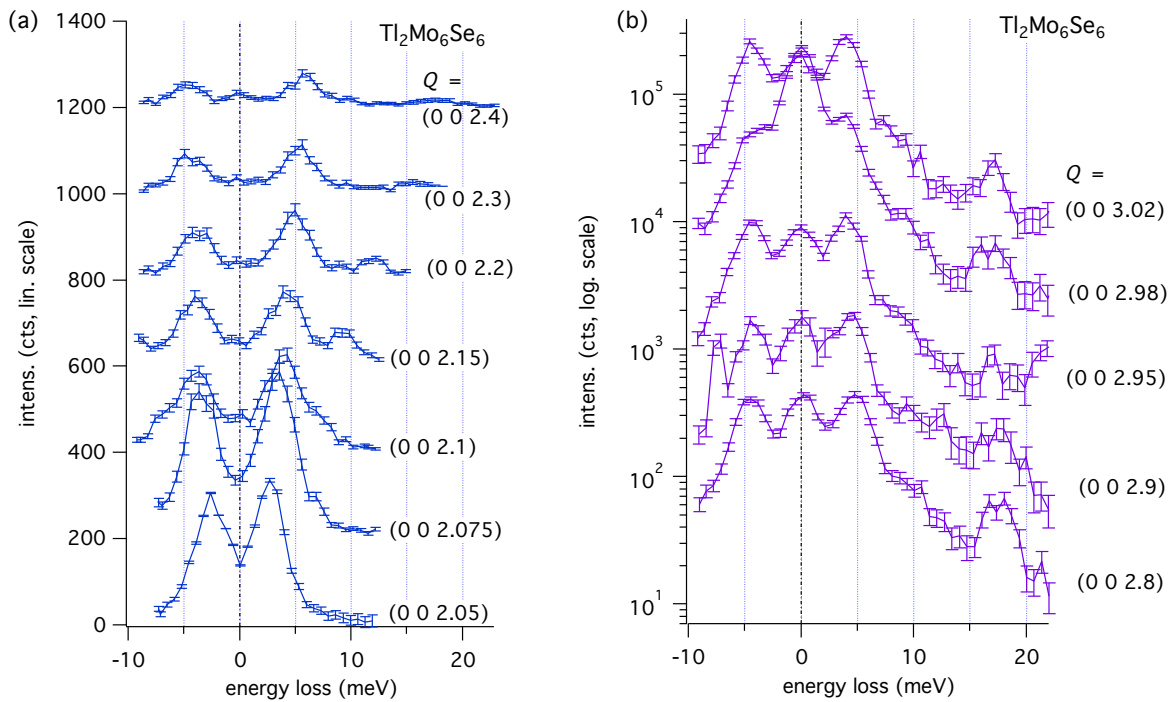
FIG. S5: Phonon spectra from \text{Tl}_2\text{Mo}_6\text{Se}_6 measured at the indicated momentum position \vec{Q} . The spectra are offset vertically for clarity.
