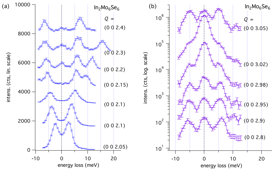
FIG. S6: Phonon spectra from \text{In}_2\text{Mo}_6\text{Se}_6 measured at the indicated momentum position \vec{Q} . The spectra are offset vertically for clarity.
