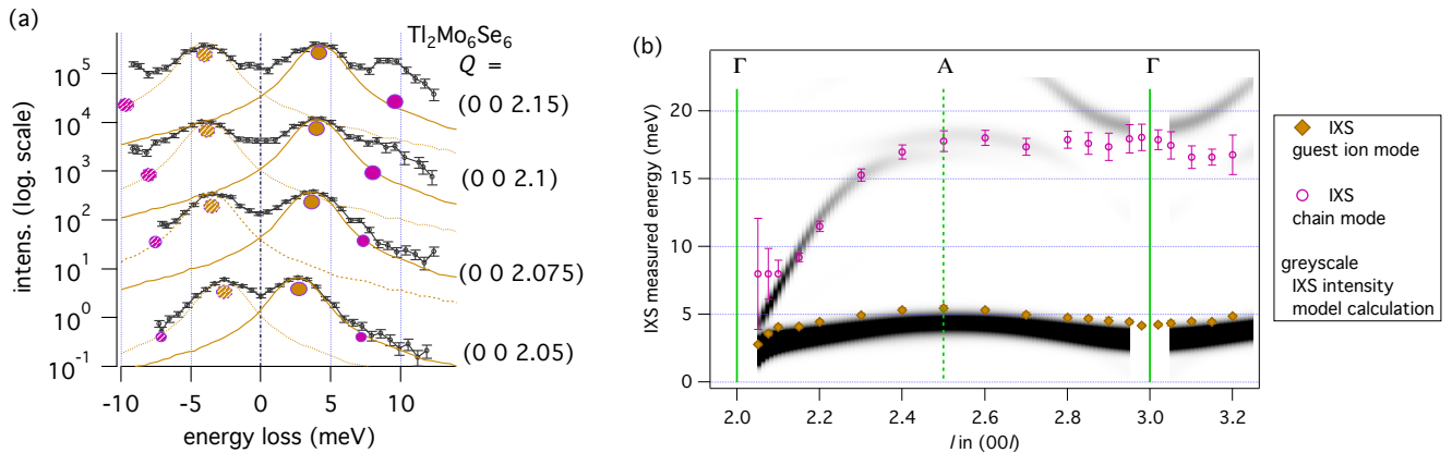
FIG. 2: (a) Selected IXS spectra of \text{Tl}_2\text{Mo}_6\text{Se}_6 close to the \Gamma -point (002). Two observed modes are indicated by brown and purple colour in solid symbols for positive energy loss and dashed symbols for negative energy loss. The resolution function, shifted to match the lowest, strongest phonon mode is shown in two copies in each spectrum. The spectra are offset vertically for graphical clarity. (b) Extracted phonon dispersions along the (00l) -direction for longitudinal modes of \text{Tl}_2\text{Mo}_6\text{Se}_6 . The data are overlaid on a grey-scale representation of the expected IXS active modes in our scattering geometry. Error bars represent the statistical uncertainty of peak positions from the numerical fits applied to the raw spectra.
