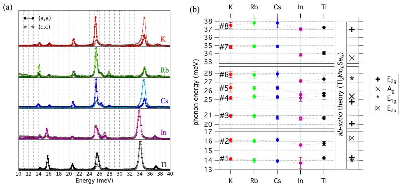
FIG. 4: (a) Raman spectroscopy of the low-energy phonon modes in the series M_2\text{Mo}_6\text{Se}_6 . Spectra with the light polarisation perpendicular and along the crystal c -axis are shown as circles and stars, respectively. (b) Peak positions of all modes observed in (a) as a function of guest ion.
