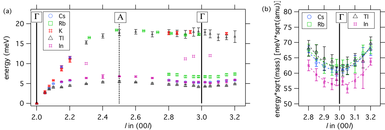
FIG. 3: (a) Longitudinal phonon dispersions for several M_2\text{Mo}_6\text{Se}_6 . (b) A comparison of the dispersion of the guest-ion modes about the \Gamma -point, normalised against the guest-ion mass.
