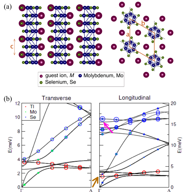
FIG. 1: (a) Crystal structure of M_2\text{Mo}_6\text{Se}_6 , seen along a (left) and along the unique axis c (right). (b) Calculated phonon dispersions for \text{Tl}_2\text{Mo}_6\text{Se}_6 . Coloured circles mark the contributions from \text{Tl} , \text{Mo} and \text{Se} for the transverse (left) and longitudinal (right) phonons. The longitudinal guest-ion and chain modes are marked by a brown and a purple arrow, respectively. Note the different energy scales for the two panels.
