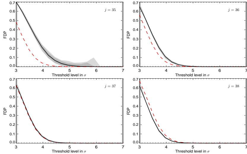
Figure 4. False Discovery Proportion: FDP as a function of threshold (in units of standard deviation) for different needlet scales. The dashed red curves are for the analytical upper bounds while the black curves are for the mean of the empirical FDPs from 100 Monte Carlo simulations. The gray shades are for percentiles 68, 95 and 99%.
