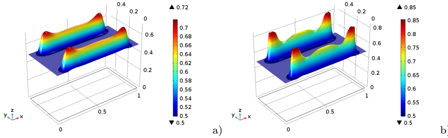
Fig. 15 Normalized mass density in non-uniform tension test with the nonlocal instantaneous model of stimulus. a) intermediate stage; b) final stage.
