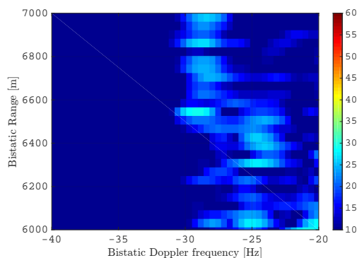
Fig. 4.24: Range-Doppler map for RpF after flex-DPCA: Enlarged view into Fig. 4.10 at the cooperative target’s position.
