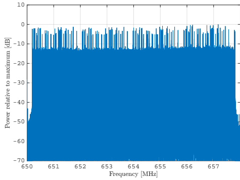
Fig. 4.5: DVB-T channel at 650 MHz. Fig. 4.6: Constellation maps for four decoded DVB-T symbols (before remapping to the constellation map). The black crosses indicate the ideal positions of the constellation points.
