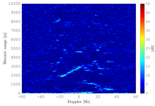
Fig. 5.34: Range-Doppler map in dB after STAP and matched filtering.
