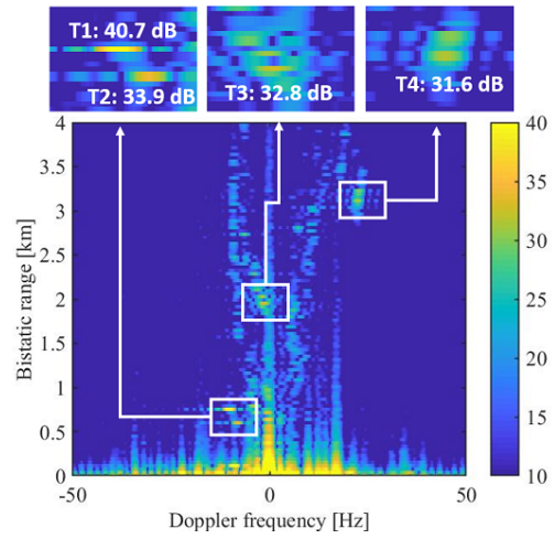
Fig. 4.10: Range Doppler map obtained for the experimental data after: STAP after RpF.
