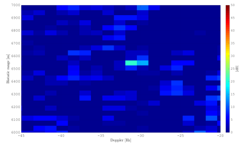
Fig. 5.37: Enlarged view for the region of the cooperative target for Fig. 5.35.
