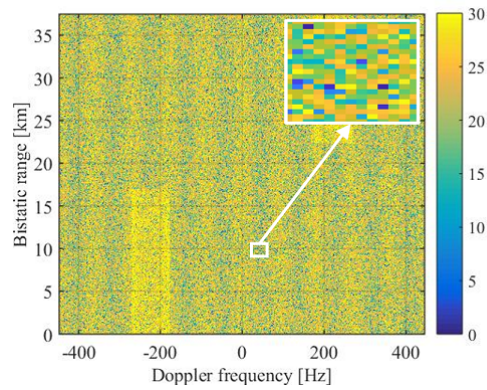
Fig. 5.5: Range-Doppler map in dB for the scenario including target, clutter, and noise with STAP being applied and MF used for range compression.
