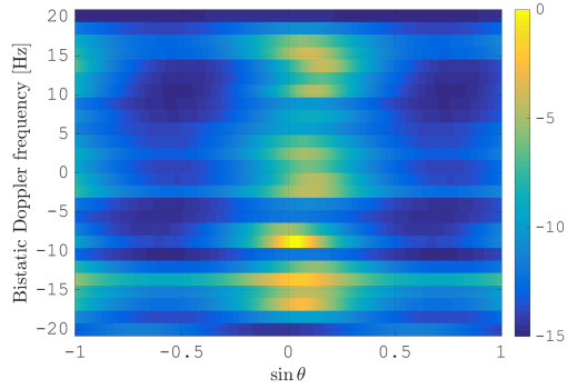
Fig. 5.26: MV power spectrum of the data from the seaborne trials after flex-DPCA and SRDB calibration.
