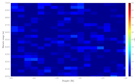
Fig. 5.36: Enlarged view for the region of the cooperative target for Fig. 5.34.
