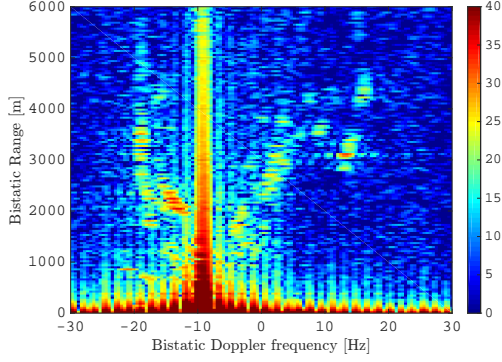
Fig. 5.17: Range-Doppler map after RpF and DPCA without calibration.
