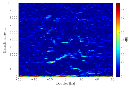
Fig. 5.35: Range-Doppler map in dB after STAP and reciprocal filtering.
