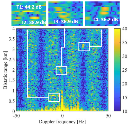
Fig. 4.9: Range Doppler map obtained for the experimental data after: STAP after MF.
