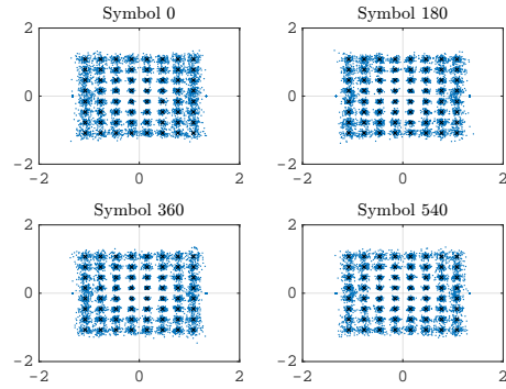
Fig. 4.5: DVB-T channel at 650 MHz. Fig. 4.6: Constellation maps for four decoded DVB-T symbols (before remapping to the constellation map). The black crosses indicate the ideal positions of the constellation points.
