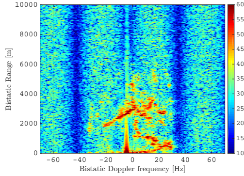
Fig. 4.21: Range-Doppler map obtained for the experimental data for MF after flex-DPCA.
