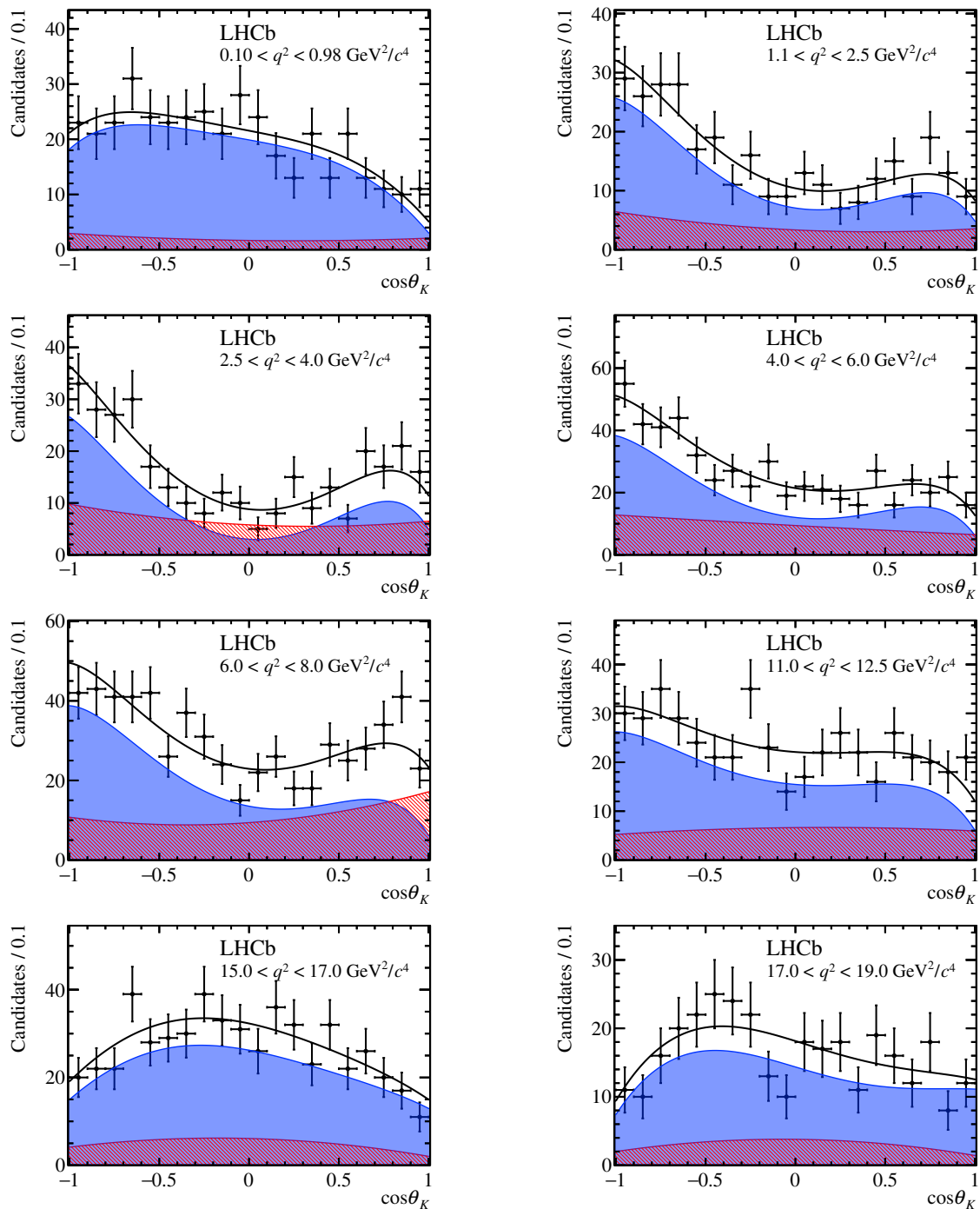
Figure 9. The \cos\theta_K angular distributions for the fine q^2 bins for candidates in the signal m_{K\pi\pi\mu} window of \pm 50 \text{ MeV}/c^2 around the known B^0 mass.
