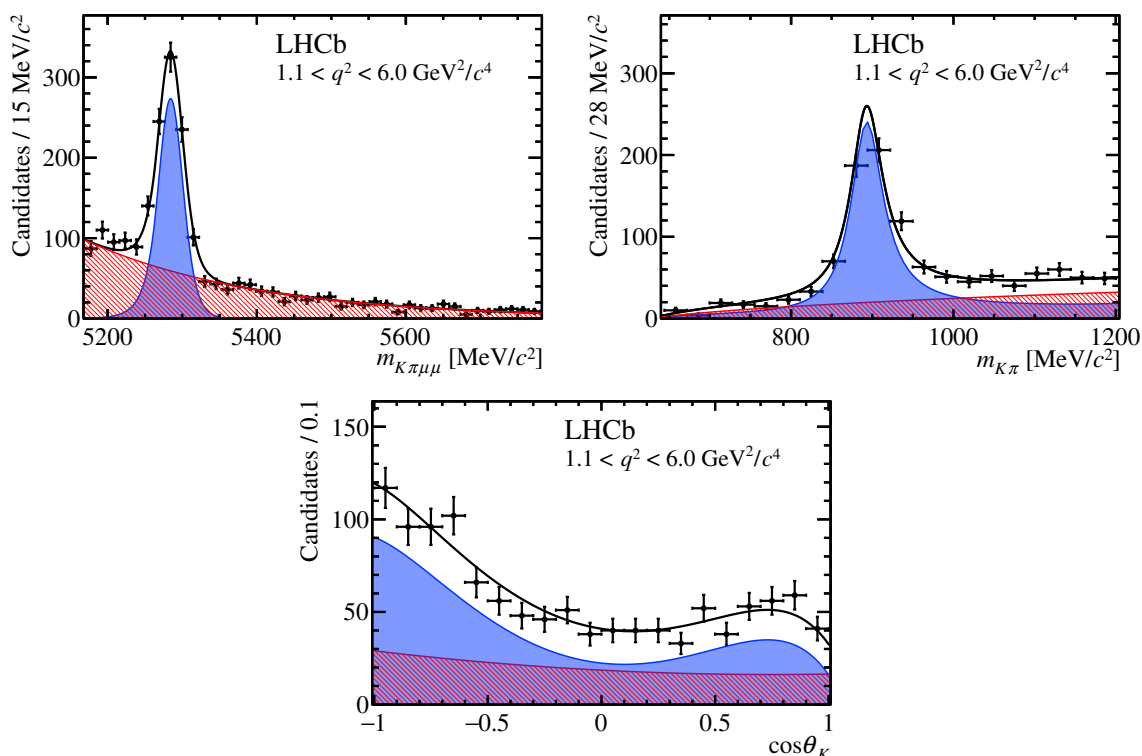
Figure 3. Angular and mass distributions for the q^2 bin 1.1 < q^2 < 6.0 \text{ GeV}^2/c^4 . The distributions of \cos\theta_K and m_{K\pi} are shown for candidates in the signal m_{K\pi\mu\mu} window of \pm 50 \text{ MeV}/c^2 around the known B^0 mass. The solid line denotes the total fitted distribution. The individual components, signal (blue shaded area) and background (red hatched area), are also shown.
