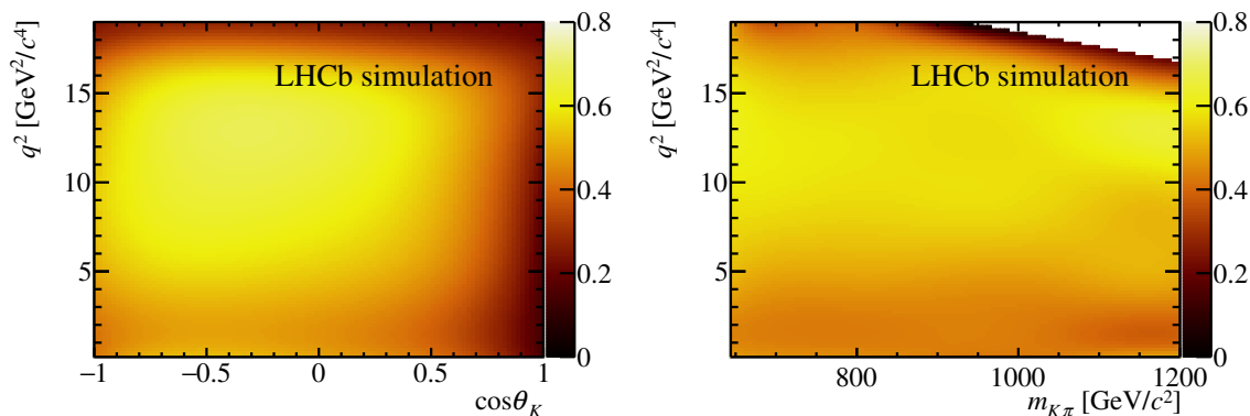
Figure 2. Two-dimensional projections of the efficiency (left) in the \cos\theta_K - q^2 plane and (right) in the m_{K\pi} - q^2 plane, determined from a principal moments analysis of simulated four-body B^0 \rightarrow K^+\pi^-\mu^+\mu^- phase-space decays. The colour scale denotes the efficiency in arbitrary units. The lack of entries in the top right corner of the m_{K\pi} - q^2 distribution is due to the limited phase space available in the decay of the B^0 meson.
