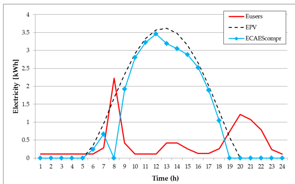
Figure 7. Daily profile: energy consumption; energy produced by PV; energy available for air compression.
