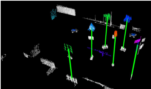
Fig. 11: A localization example in the map illustrated in Fig. 9. Segments extracted from the target map are shown in white below whereas colors are used to depict segments extracted from the local representation of the robot located at the right. Matching segments resulting in a localization are illustrated with vertical green lines.
