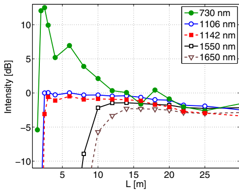
Fig. 3. Longitudinal evolution of the spectral intensity at selected spectral components from Fig. 2.
