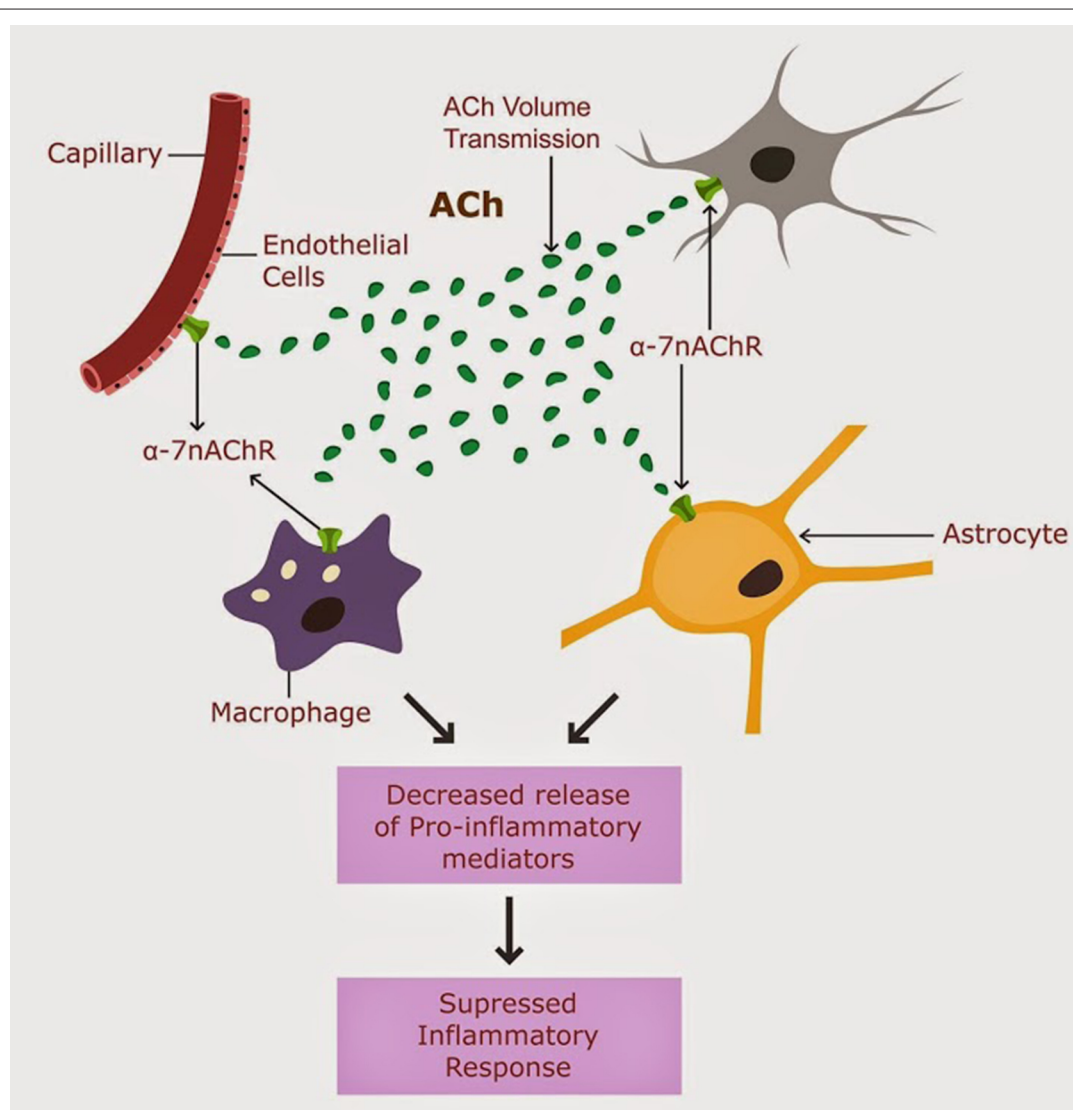
FIGURE 1 | CAIS is operational in the CNS, and involves ACh action of alpha 7 nAChRs expressed on astrocytes, neurons, microglia and brain macrophages (Tyagi et al., 2010).
