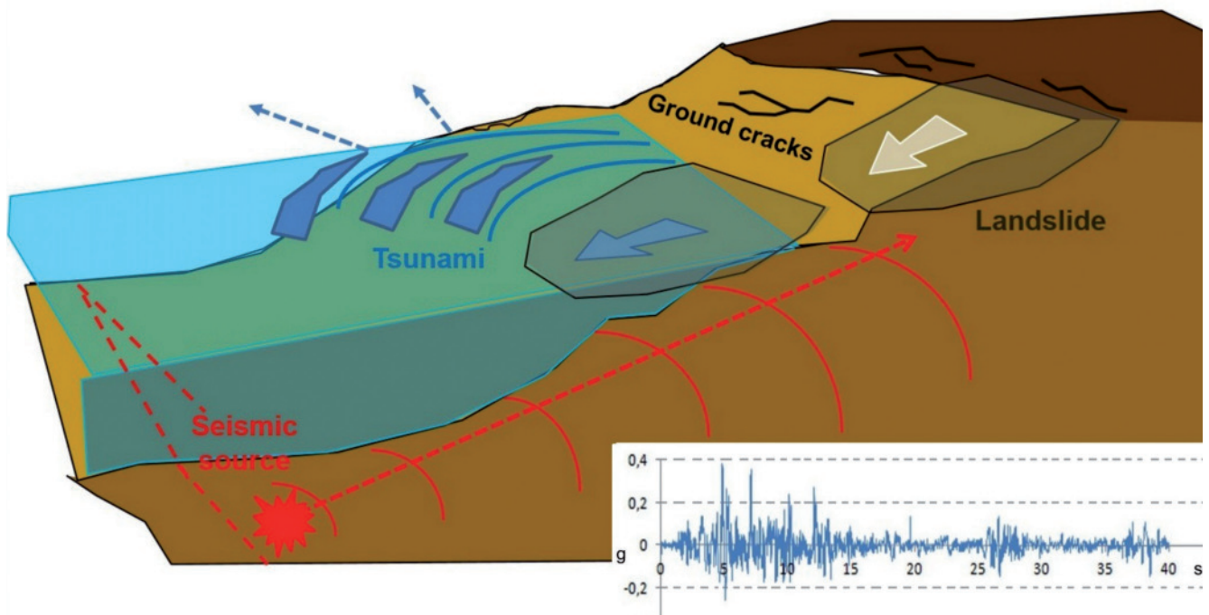
Fig. 2 - Earthquake-induced landslides can be regarded as part of a “domino effect” since they are triggered by an action external respect to the slope. However, they can also cause other effects, such as tsunamis
