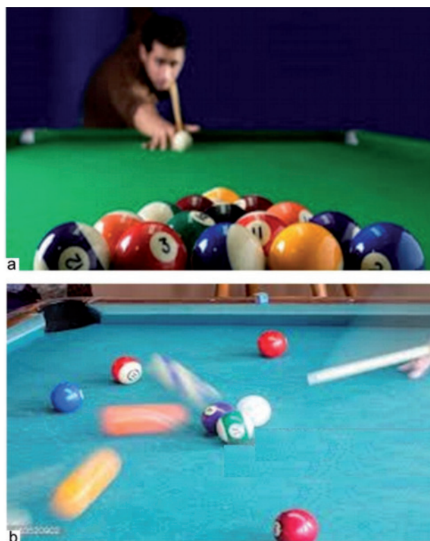
Fig. 1 - Risk perspective for multi-hazard. a) a single hazardous event can threaten many exposed subjects (human and/or natural); b) a single a hazardous event can trigger several phenomena by a “domino effect”, i.e. a concatenated sequence of effects
