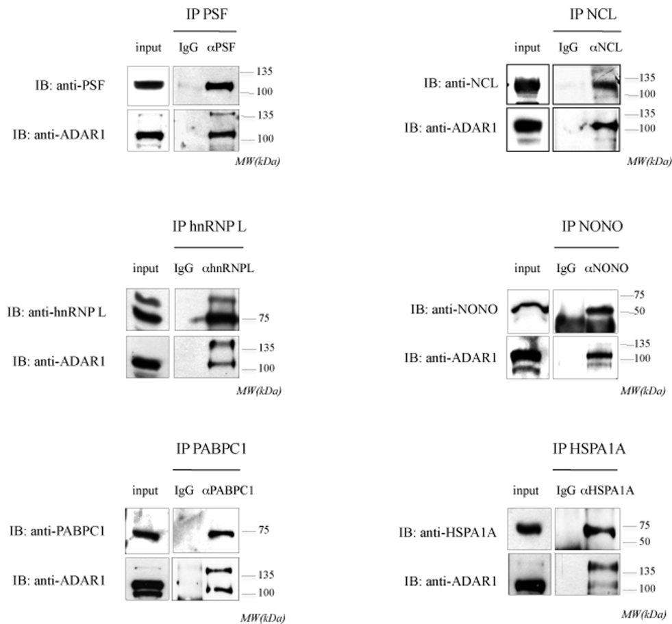
Figure 3. Validation of the results of the nano-LC MS/MS data by reciprocal IP. Lysate of 293T cells was subjected to IP using either IgGs or anti-NONO or anti-PSF or anti-hnRNP L or anti-NCL or anti-HSPA1A or anti-PABPC1 antibodies followed by WB analysis using specific antibodies. WB analysis of 20 \mu g of cell lysate inputs (input) is shown.
