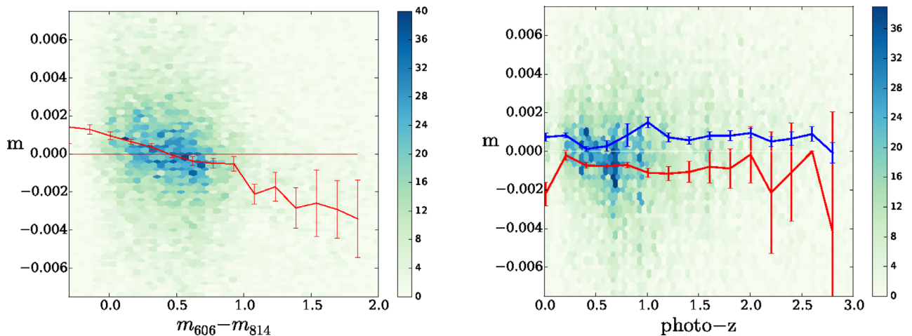
Figure 13. Multiplicative CG bias as a function of observed colour ( m_{606} - m_{814} ; left-hand panel) and redshift (right-hand panel). We observe a clear trend of the average bias with colour (indicated by the red points with error bars in the left-hand panel). In the right-hand panel we split the sample into red ( m_{606} - m_{814} > 0.5 ; red line) and blue ( m_{606} - m_{814} < 0.5 ; blue line) galaxies. The variation with redshift is weak for both samples. The colour of hexagon stands for the number of galaxies.
