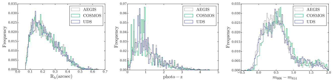
Figure 10. Histogram of the distributions in observed half-light radii ( R_h ; left-hand panel), photometric redshift (middle panel), and m_{606} - m_{814} colour (right-hand panel) for the three CANDELS fields (AEGIS, COSMOS, and UDS). We show results for galaxies with m_{VIS} < 25 , where the results for the three fields are normalized by area.
