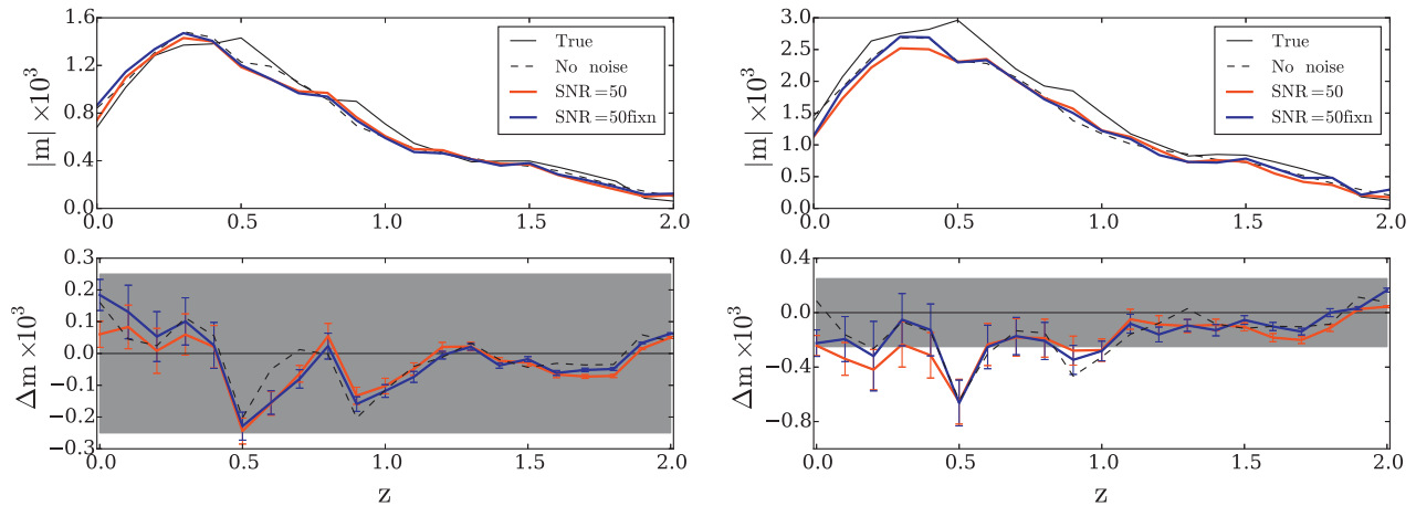
Figure 5. The multiplicative CG bias as a function of redshift for the reference galaxies, with the results for galaxy ‘B’ shown in the left-hand panel and those for galaxy ‘S’ in the right-hand panel. The dashed black line is the recovered bias when we mimic noiseless HST observations in two filters. The solid red line indicates the results when we use the best-fitting GALFIT model in both filters to estimate the CG bias when the simulated HST images have an input SNR = 50 (averaged over 40 noise realizations at each redshift). The blue line shows the results when we fix the Sérsic index in the fit. The bottom panels show the residuals \Delta m with respect to the true CG bias. The grey band indicates the nominal Euclid requirement for the residual CG bias after correction.
