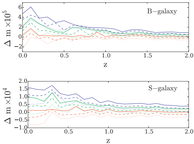
Figure 8. Change in multiplicative CG bias when the size of the PSF used in the deconvolution of the narrow-band images is increased (the FWHM differs by 5 per cent between steps). From red, green to blue lines, we increase the size of the PSF for the F814W filter; from the solid, dashed to dotted lines we increase the size of the PSF for the F606W images.
