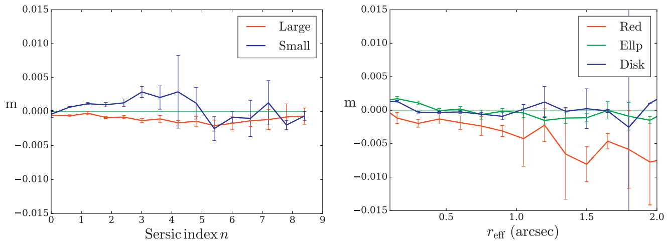
Figure 14. CG bias with Sérsic index (left) and effective radius (right) from the mock VIS images. In the left-hand panel, the blue (red) is the average of small (big) galaxies. In the right-hand panel, the red line is the average bias of red galaxies ( m_{606} - m_{814} > 1 ); the green line is that of elliptical galaxies ( n > 2.75 ); and the blue line is for the disc galaxies.
