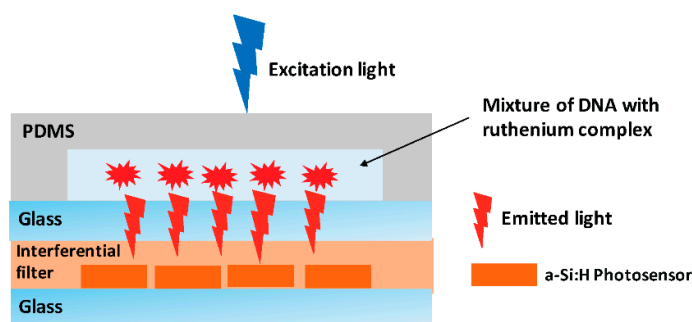
Figure 2. Schematic cross section of the structure for the on-chip detection of DNA. The thicknesses of the interferential filter is a few tens of microns. The thickness of each glass is 1 mm.
