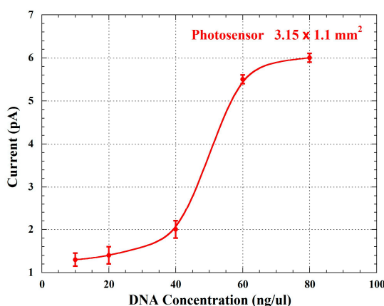
Figure 3. Sensor photocurrents as a function of the DNA concentration in the solution inside the microfluidic channel. Concentration of ruthenium complex is 6 \times 10^{-5} M. Symbols and error bars represent the averaged values and standard deviations over three independent measurements, respectively.
