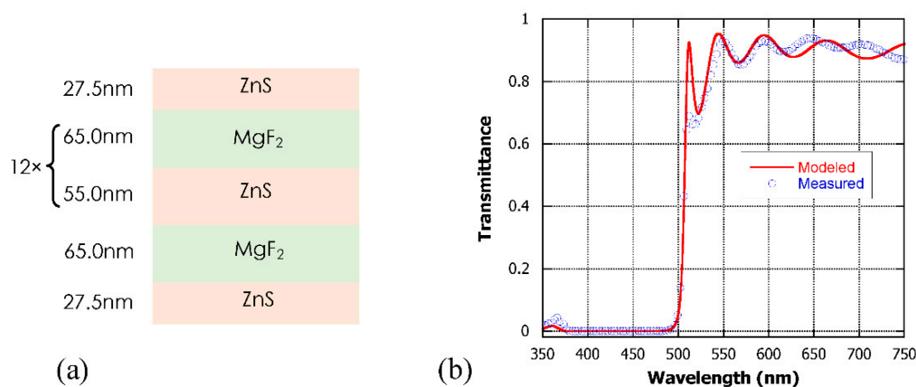
Figure 1. (a) Cross section of the interferential filter structure. (b) Modeled and measured transmittance of the filter deposited on a plain glass substrate.
