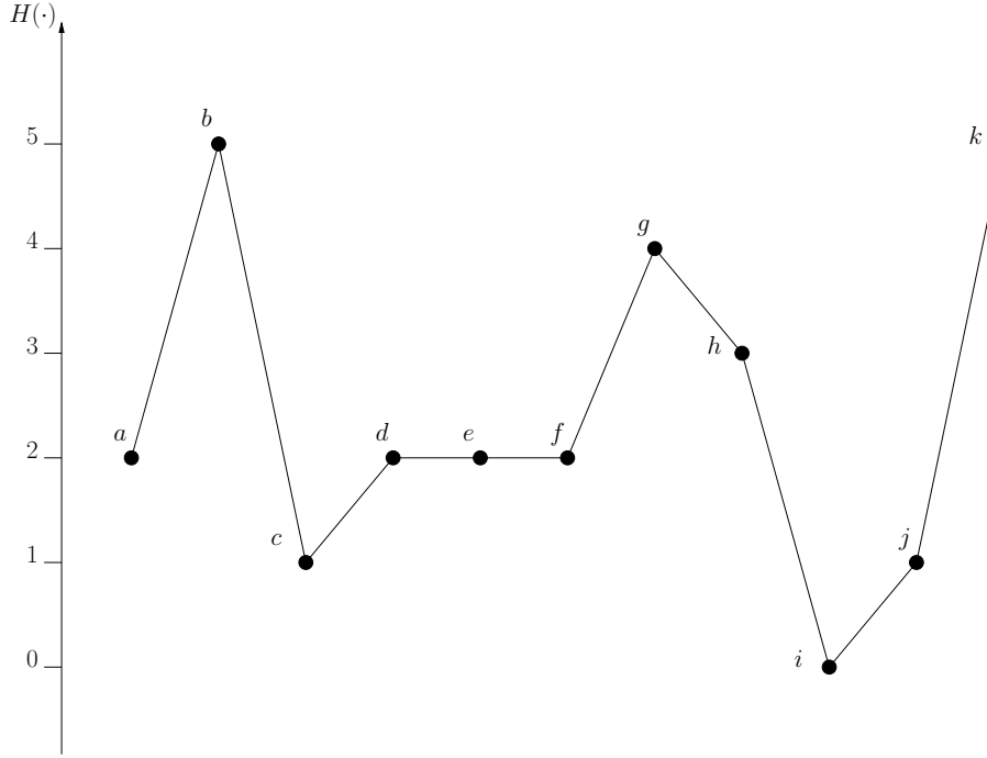
Figure 1: The energy landscape on S = \{a, b, c, d, e, f, g, h, i, j, k\}
