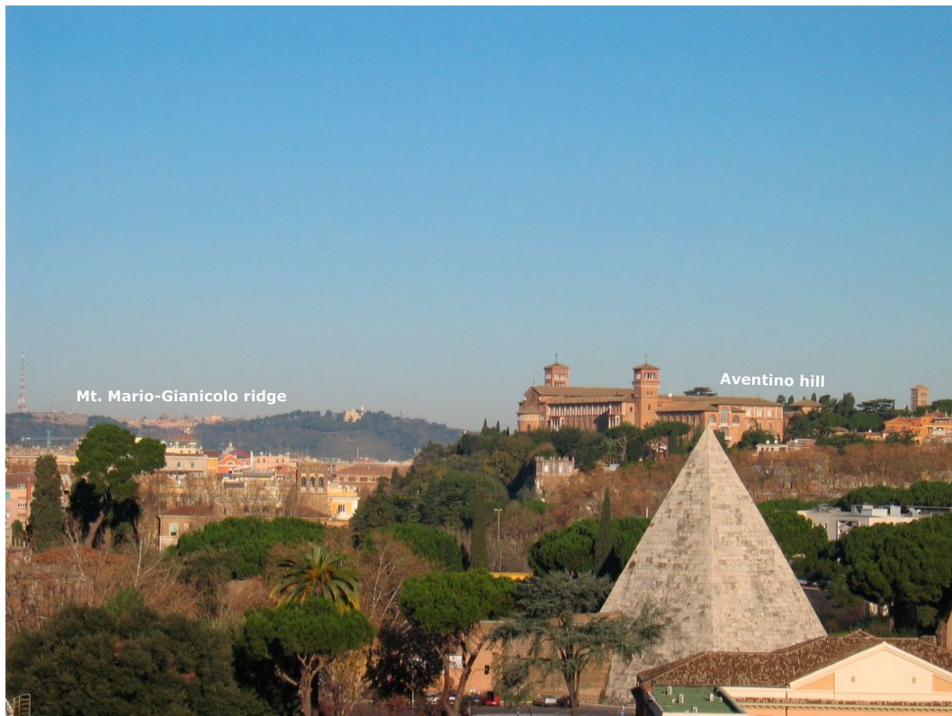
Figure 3. On the right, the southern slope of Aventino, one of the ‘Seven Hills’ that has steep slopes and a flat top, overlooking the floodplain of the Tiber. The landscape on the West side of the Tiber (left, in the background) is characterized by the Mt. Mario-Gianicolo ridge, which is higher, rugged and frequently subjected to landsliding. In the foreground, the only ancient pyramid surviving in Rome (built about 2000 years ago).
