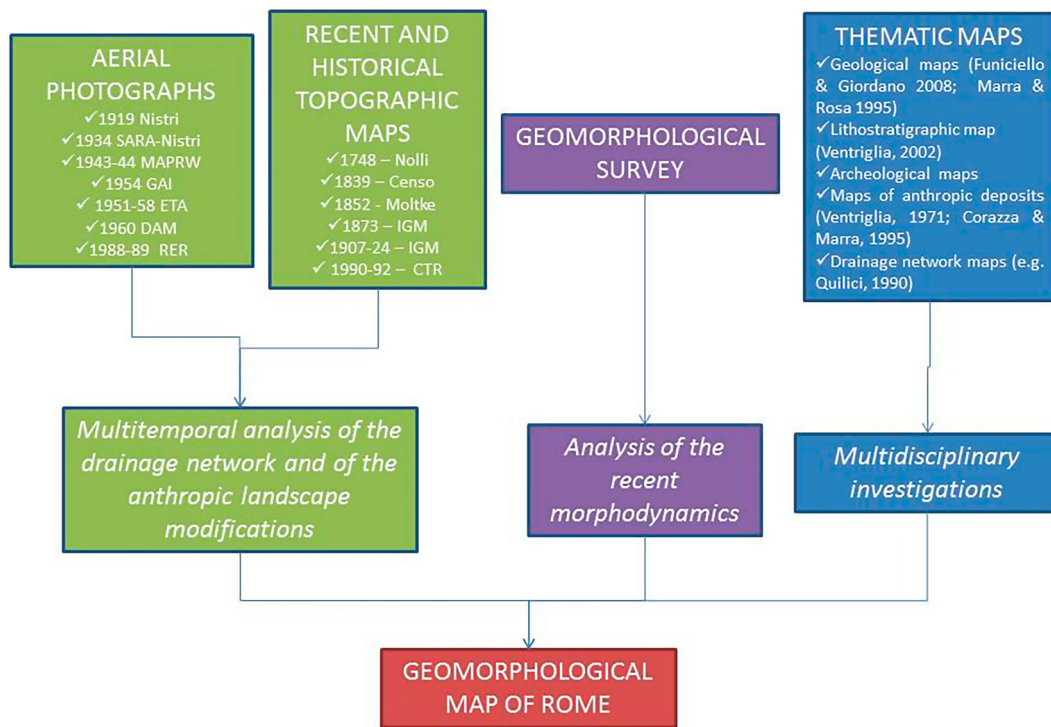
Figure 2. Flow chart summarizing the methodology used for the production of the Main Map . Only a partial list of the examined literature sources is shown.
