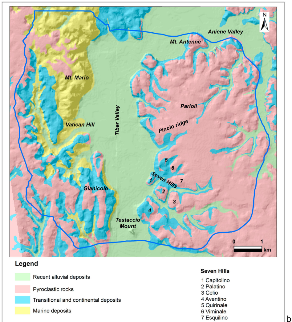
Figure 1. (a) Geological sketch of the Latium region. Modified from Del Monte et al. (2013). (b) Geological sketch of the study area. The geological sketch of Rome city centre was mainly developed comparing the 'Lithostratigraphic map' by Ventriglia (2002) with the geological maps by Funciello and Giordano (2008) and Marra and Rosa (1995).
