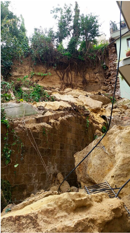
Figure 4. Rock toppling which occurred in via dell'Ongaro, Monteverde neighbourhood, in March 2015.
