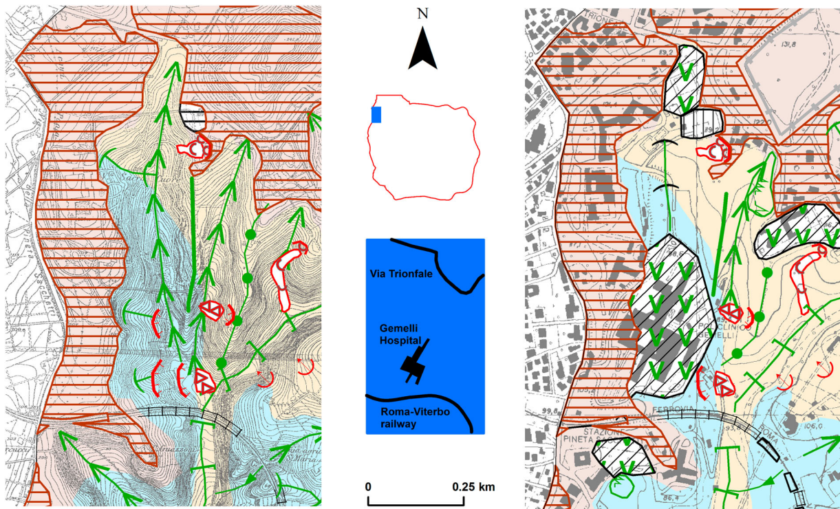
Figure 5. Multitemporal analysis of the anthropogenic modifications of the drainage network and landslide processes that occurred in the Gemelli Hospital area. In (a) the rural landscape in 1924 (IGM Piano Topografico di Roma); in (b) the present-day situation (CTR Lazio 374060–374070). This area is characterized by several valleys that have been heavily modified due to urbanization; some of them were previously affected by landslides. The figure highlights that in 1924 the selected area was characterized by natural landforms, including fluvial valleys (green), landslides (red) and structural surfaces (brown). Currently some man-made landforms (black) have been superimposed on natural landforms, such as filling material in ancient valleys; other natural landforms were partially buried and reduced in extent. A more detailed description of the landforms represented can be found in the legend of the Main Map.
